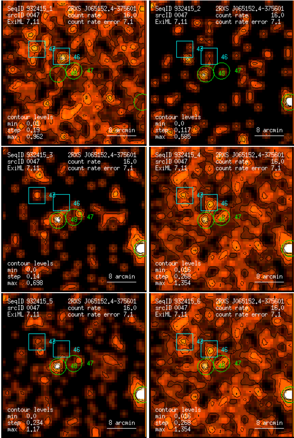
Figure 47: RASS 932415: detection 0047: band rate images, Gaussian filter: (1) PSPC channels 11 – 41, (2) 52 – 90, (3) 91 – 201, (4) 11 – 235, (5) 52 – 201, (6) 11 – 201. Broad band rates in counts/ks. Band rate contour levels in counts/ks/arcmin 2 .
