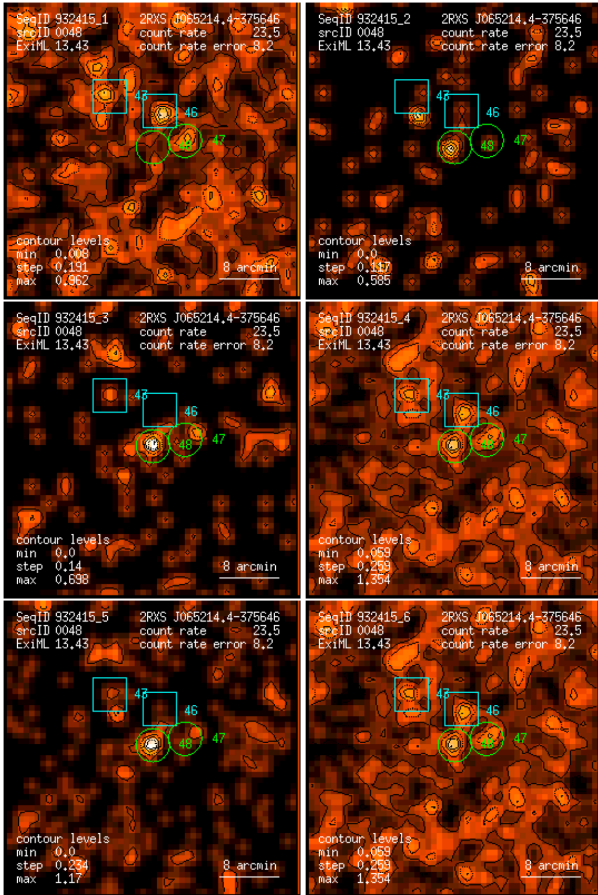
Figure 48: RASS 932415: detection 0048: band rate images, Gaussian filter: (1) PSPC channels 11 – 41, (2) 52 – 90, (3) 91 – 201, (4) 11 – 235, (5) 52 – 201, (6) 11 – 201. Broad band rates in counts/ks. Band rate contour levels in counts/ks/arcmin 2 .
