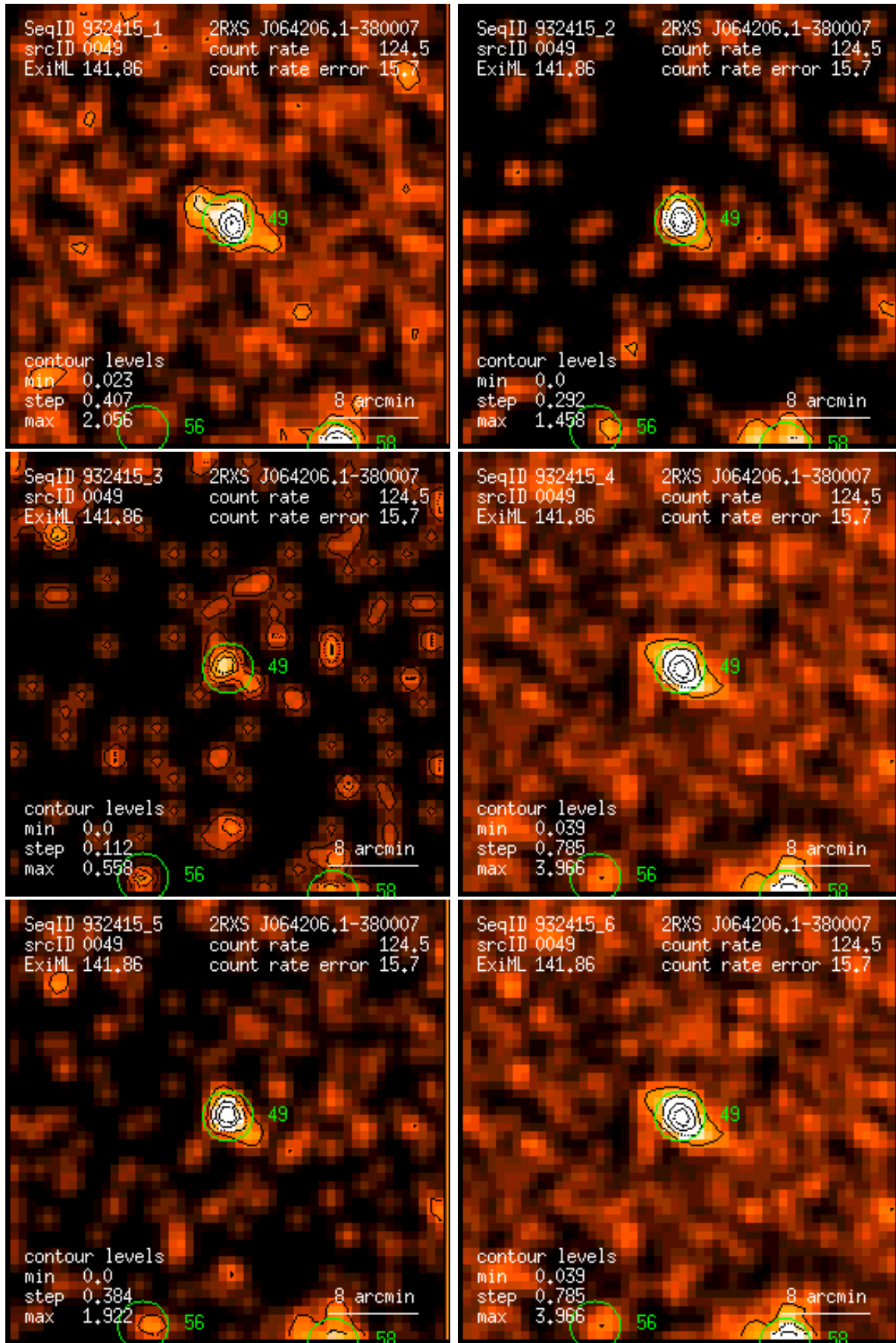
Figure 49: RASS 932415: detection 0049: band rate images, Gaussian filter: (1) PSPC channels 11 – 41, (2) 52 – 90, (3) 91 – 201, (4) 11 – 235, (5) 52 – 201, (6) 11 – 201. Broad band rates in counts/ks. Band rate contour levels in counts/ks/arcmin 2 .
