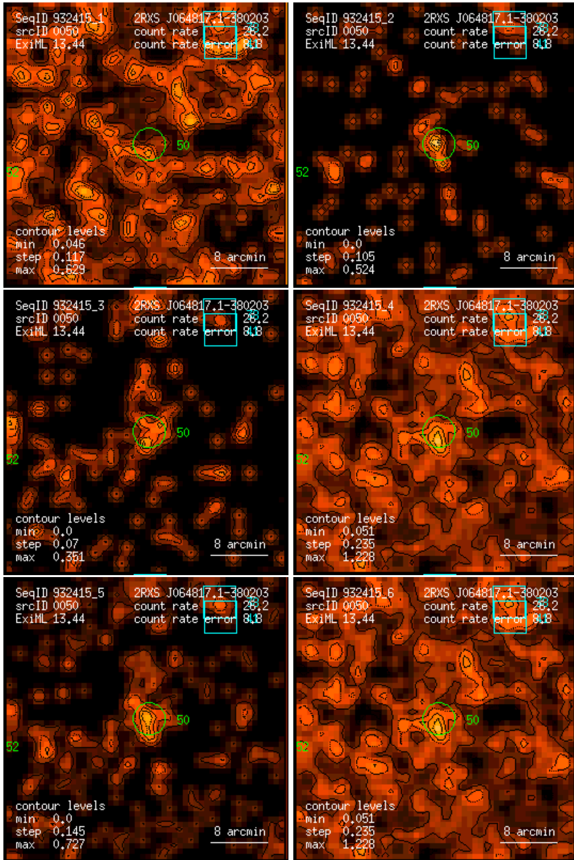
Figure 50: RASS 932415: detection 0050: band rate images, Gaussian filter: (1) PSPC channels 11 – 41, (2) 52 – 90, (3) 91 – 201, (4) 11 – 235, (5) 52 – 201, (6) 11 – 201. Broad band rates in counts/ks. Band rate contour levels in counts/ks/arcmin 2 .
