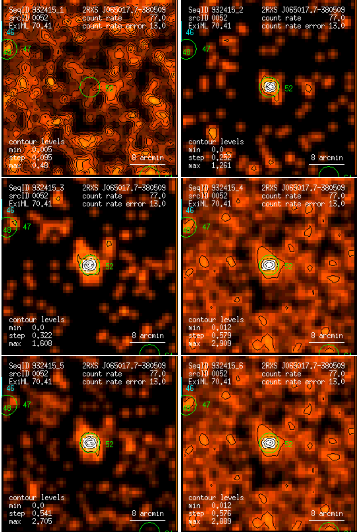
Figure 52: RASS 932415: detection 0052: band rate images, Gaussian filter: (1) PSPC channels 11 – 41, (2) 52 – 90, (3) 91 – 201, (4) 11 – 235, (5) 52 – 201, (6) 11 – 201. Broad band rates in counts/ks. Band rate contour levels in counts/ks/arcmin 2 .
