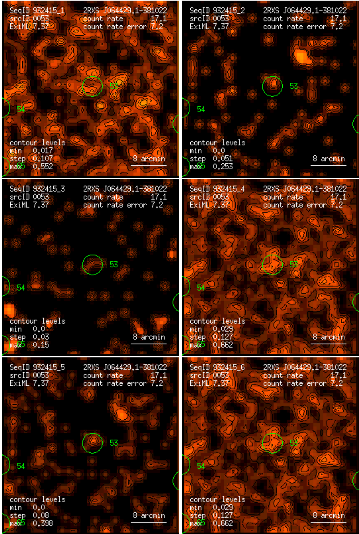
Figure 53: RASS 932415: detection 0053: band rate images, Gaussian filter: (1) PSPC channels 11 – 41, (2) 52 – 90, (3) 91 – 201, (4) 11 – 235, (5) 52 – 201, (6) 11 – 201. Broad band rates in counts/ks. Band rate contour levels in counts/ks/arcmin 2 .
