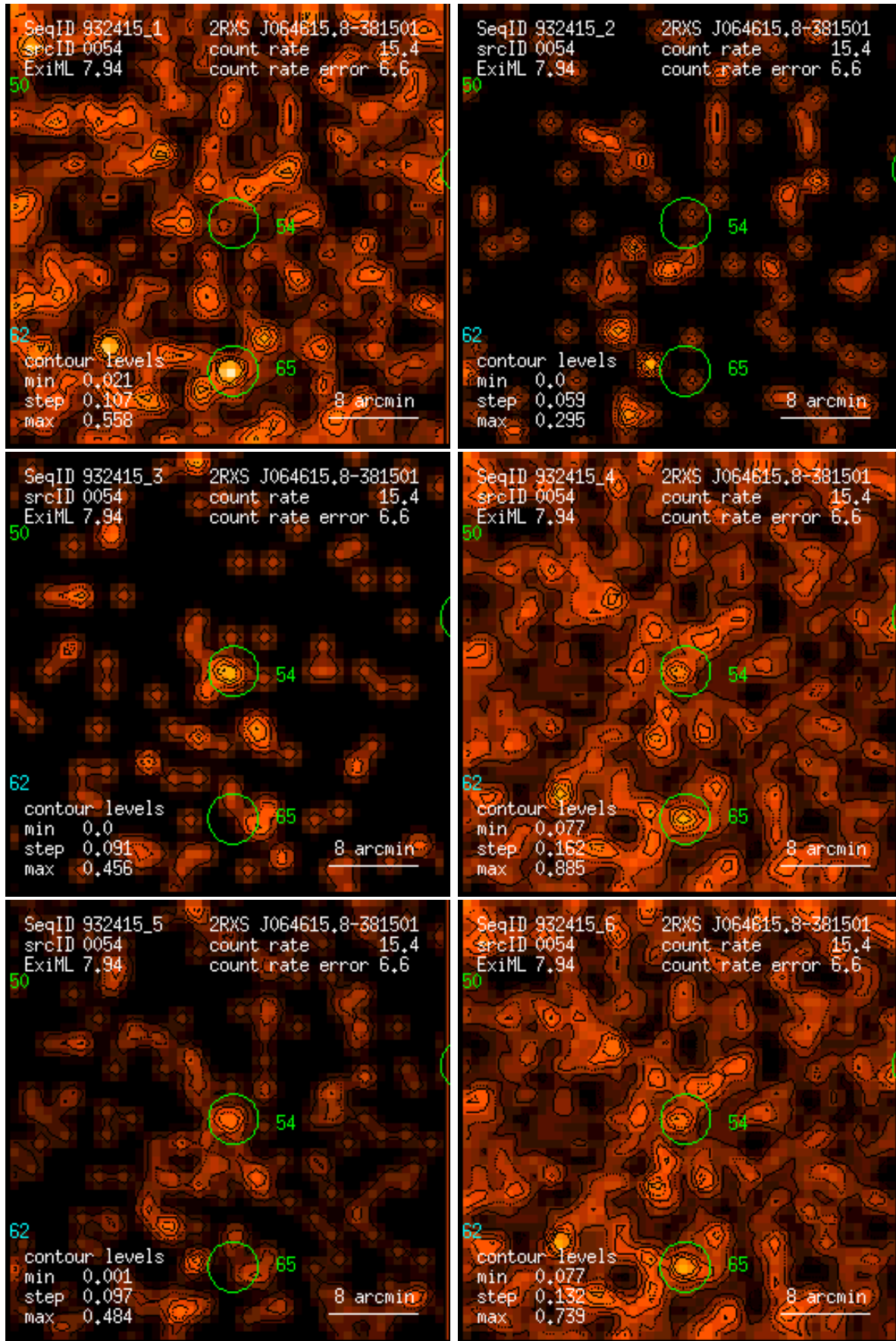
Figure 54: RASS 932415: detection 0054: band rate images, Gaussian filter: (1) PSPC channels 11 – 41, (2) 52 – 90, (3) 91 – 201, (4) 11 – 235, (5) 52 – 201, (6) 11 – 201. Broad band rates in counts/ks. Band rate contour levels in counts/ks/arcmin 2 .
