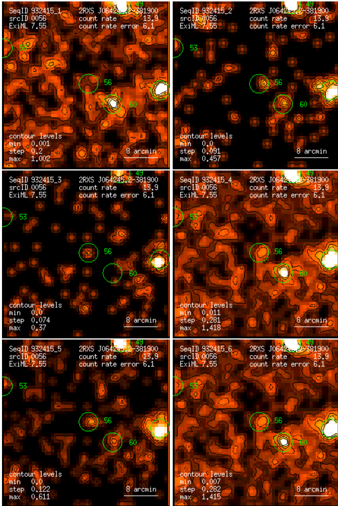
Figure 56: RASS 932415: detection 0056: band rate images, Gaussian filter: (1) PSPC channels 11 – 41, (2) 52 – 90, (3) 91 – 201, (4) 11 – 235, (5) 52 – 201, (6) 11 – 201. Broad band rates in counts/ks. Band rate contour levels in counts/ks/arcmin 2 .
