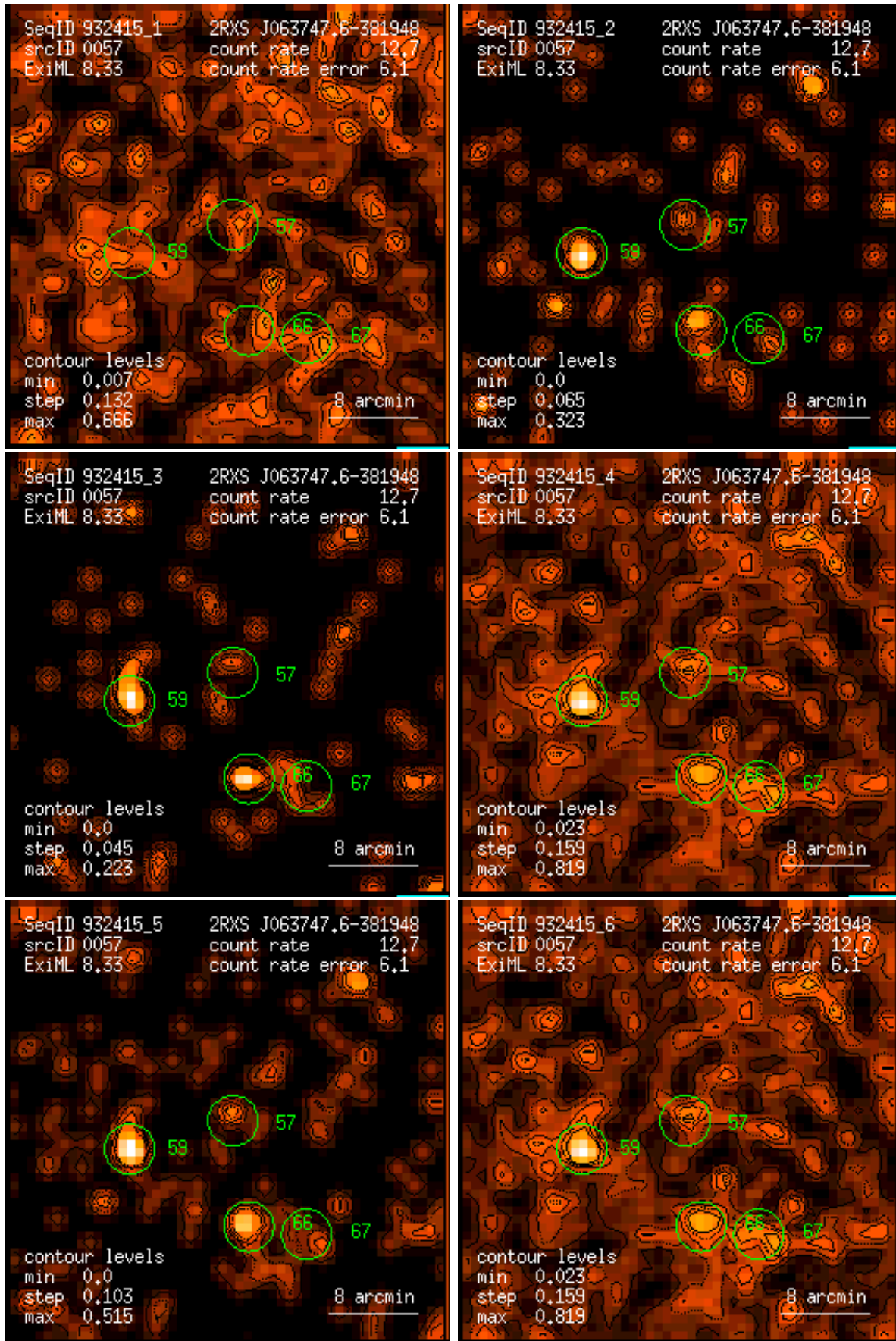
Figure 57: RASS 932415: detection 0057: band rate images, Gaussian filter: (1) PSPC channels 11 – 41, (2) 52 – 90, (3) 91 – 201, (4) 11 – 235, (5) 52 – 201, (6) 11 – 201. Broad band rates in counts/ks. Band rate contour levels in counts/ks/arcmin 2 .
