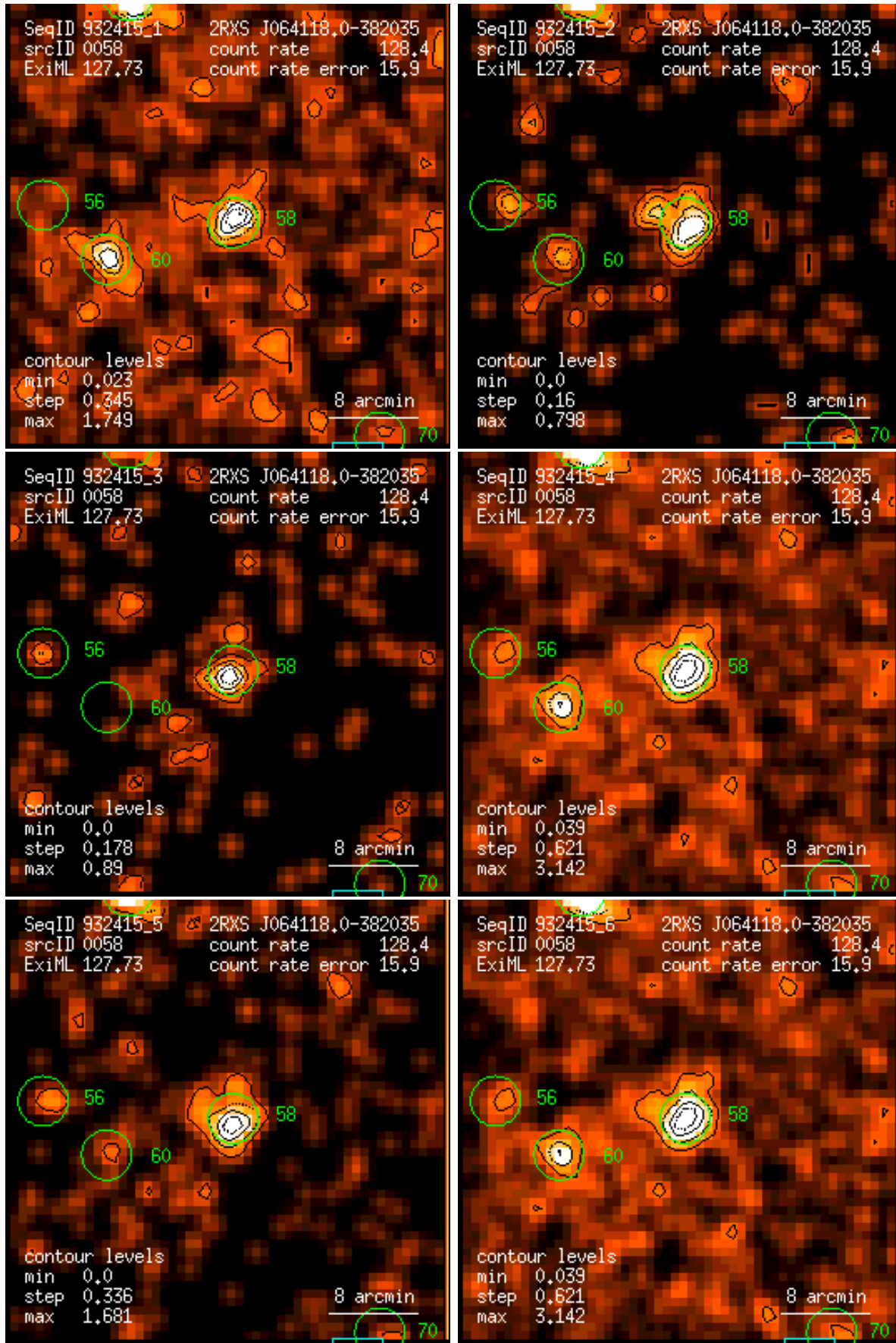
Figure 58: RASS 932415: detection 0058: band rate images, Gaussian filter: (1) PSPC channels 11 – 41, (2) 52 – 90, (3) 91 – 201, (4) 11 – 235, (5) 52 – 201, (6) 11 – 201. Broad band rates in counts/ks. Band rate contour levels in counts/ks/arcmin 2 .
