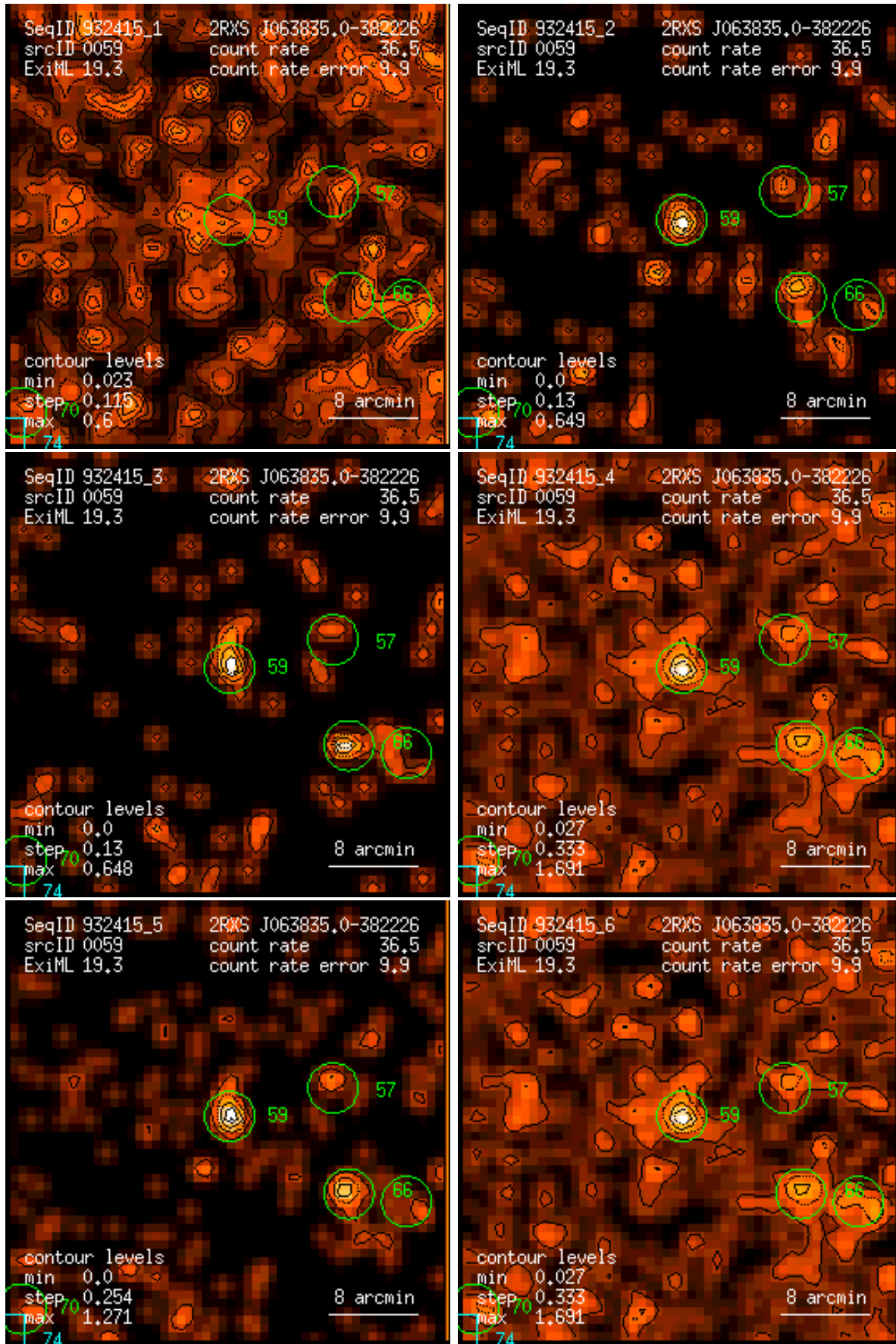
Figure 59: RASS 932415: detection 0059: band rate images, Gaussian filter: (1) PSPC channels 11 – 41, (2) 52 – 90, (3) 91 – 201, (4) 11 – 235, (5) 52 – 201, (6) 11 – 201. Broad band rates in counts/ks. Band rate contour levels in counts/ks/arcmin 2 .
