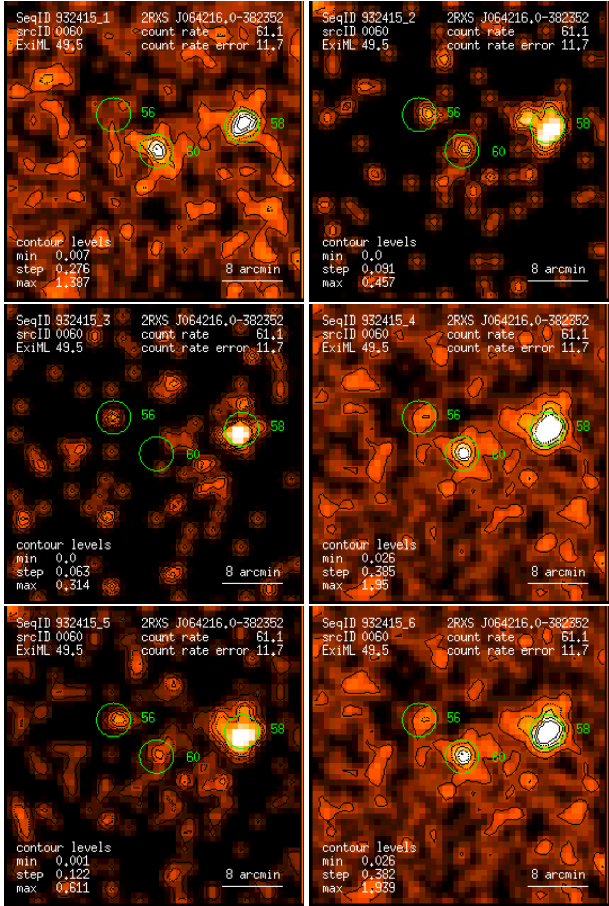
Figure 60: RASS 932415: detection 0060: band rate images, Gaussian filter: (1) PSPC channels 11 – 41, (2) 52 – 90, (3) 91 – 201, (4) 11 – 235, (5) 52 – 201, (6) 11 – 201. Broad band rates in counts/ks. Band rate contour levels in counts/ks/arcmin 2 .
