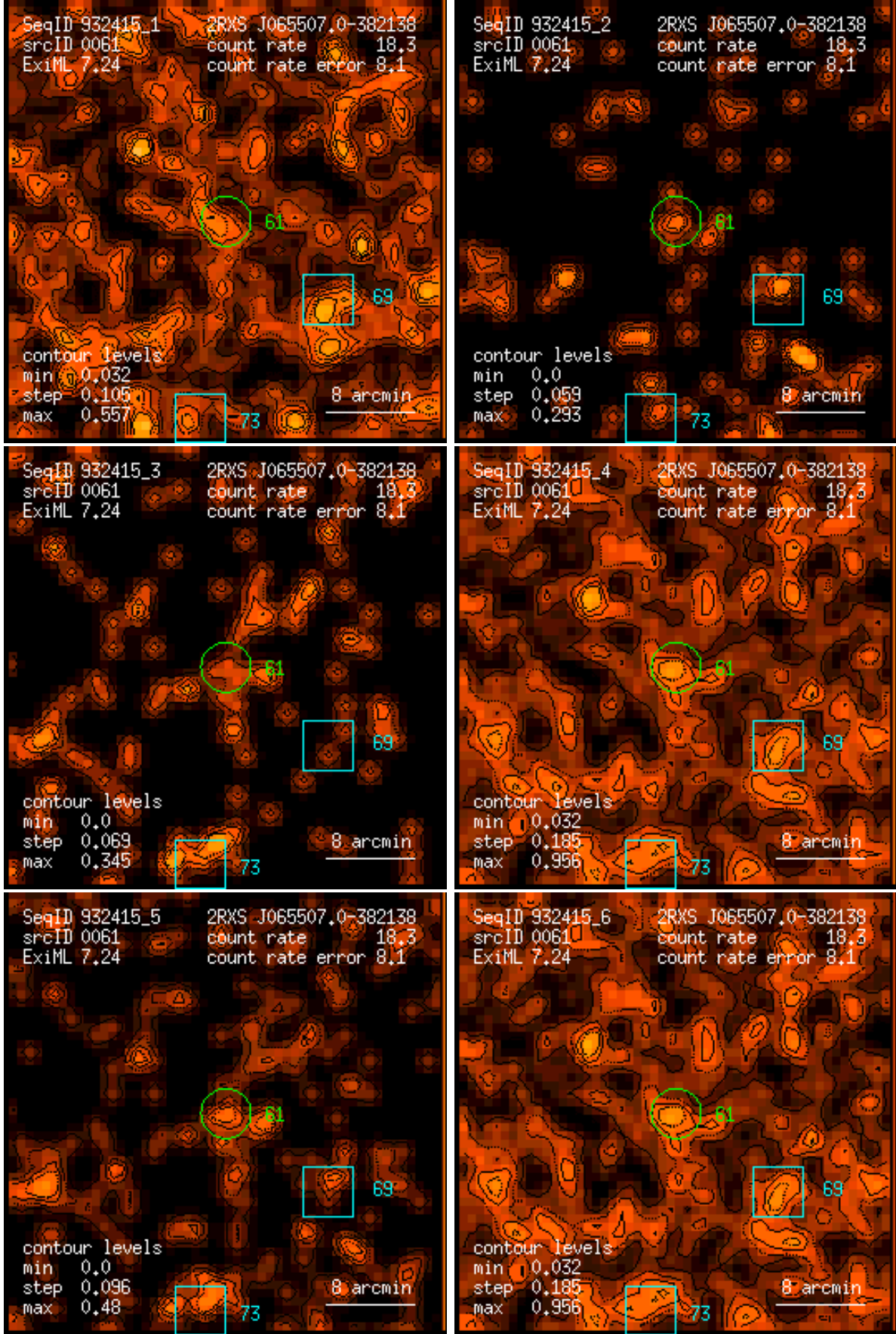
Figure 61: RASS 932415: detection 0061: band rate images, Gaussian filter: (1) PSPC channels 11 – 41, (2) 52 – 90, (3) 91 – 201, (4) 11 – 235, (5) 52 – 201, (6) 11 – 201. Broad band rates in counts/ks. Band rate contour levels in counts/ks/arcmin 2 .
