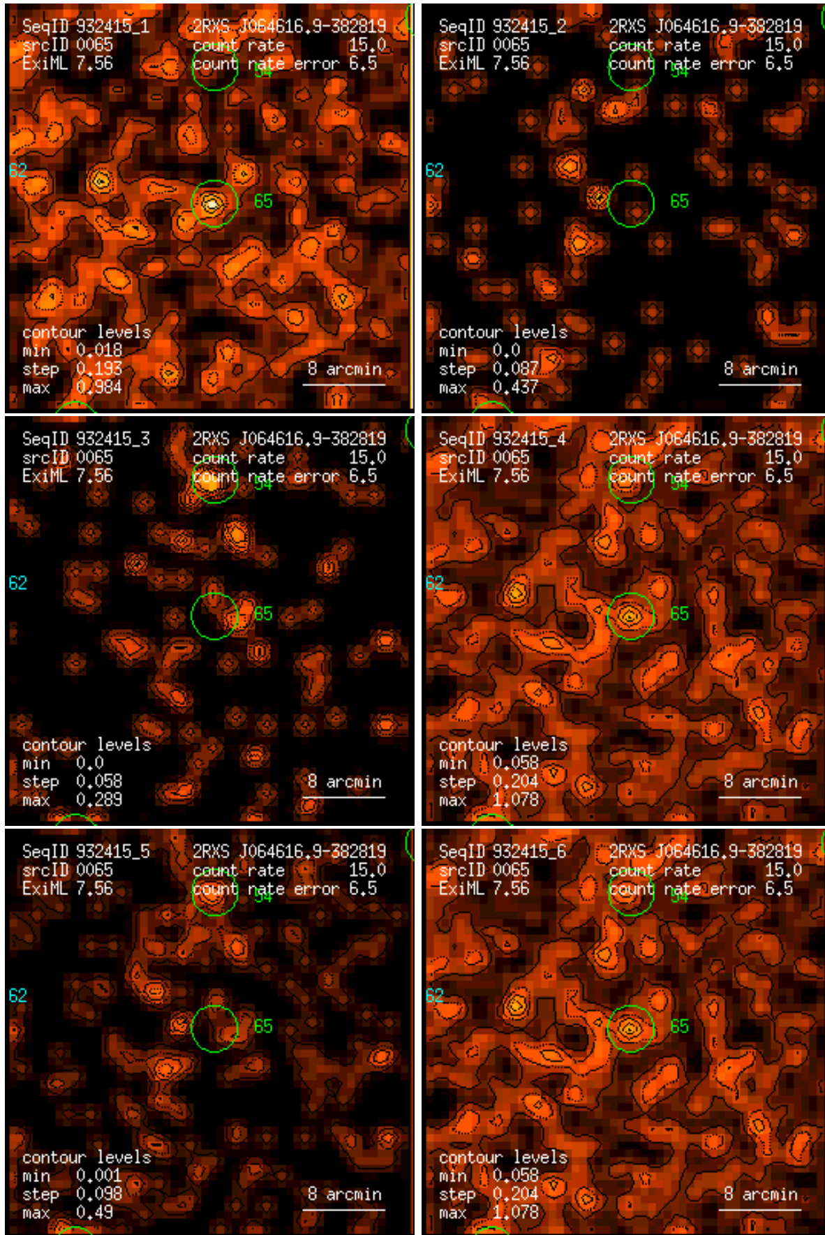
Figure 65: RASS 932415: detection 0065: band rate images, Gaussian filter: (1) PSPC channels 11 – 41, (2) 52 – 90, (3) 91 – 201, (4) 11 – 235, (5) 52 – 201, (6) 11 – 201. Broad band rates in counts/ks. Band rate contour levels in counts/ks/arcmin 2 .
