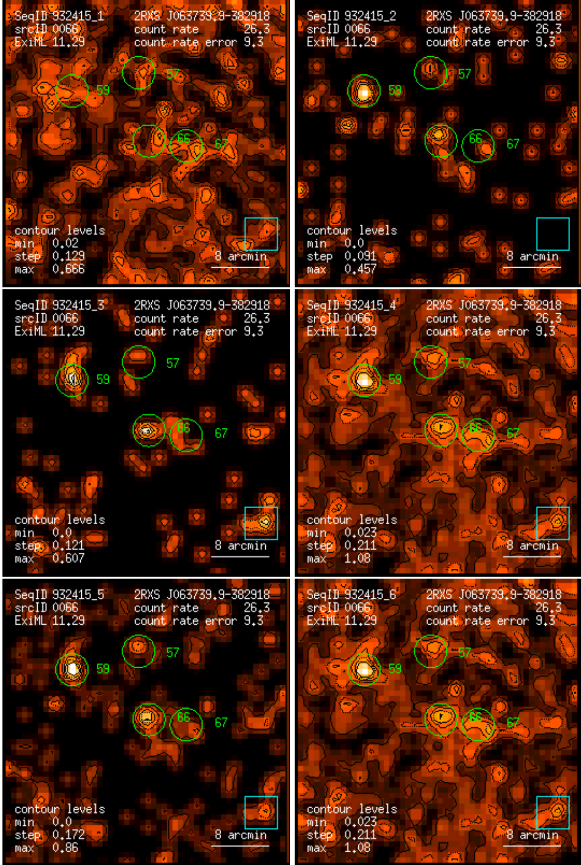
Figure 66: RASS 932415: detection 0066: band rate images, Gaussian filter: (1) PSPC channels 11 – 41, (2) 52 – 90, (3) 91 – 201, (4) 11 – 235, (5) 52 – 201, (6) 11 – 201. Broad band rates in counts/ks. Band rate contour levels in counts/ks/arcmin 2 .
