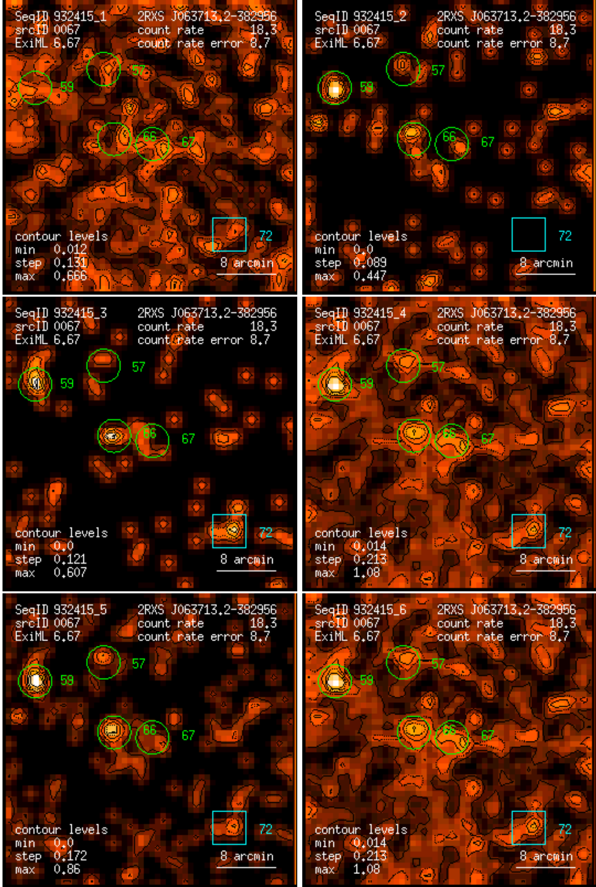
Figure 67: RASS 932415: detection 0067: band rate images, Gaussian filter: (1) PSPC channels 11 – 41, (2) 52 – 90, (3) 91 – 201, (4) 11 – 235, (5) 52 – 201, (6) 11 – 201. Broad band rates in counts/ks. Band rate contour levels in counts/ks/arcmin 2 .
