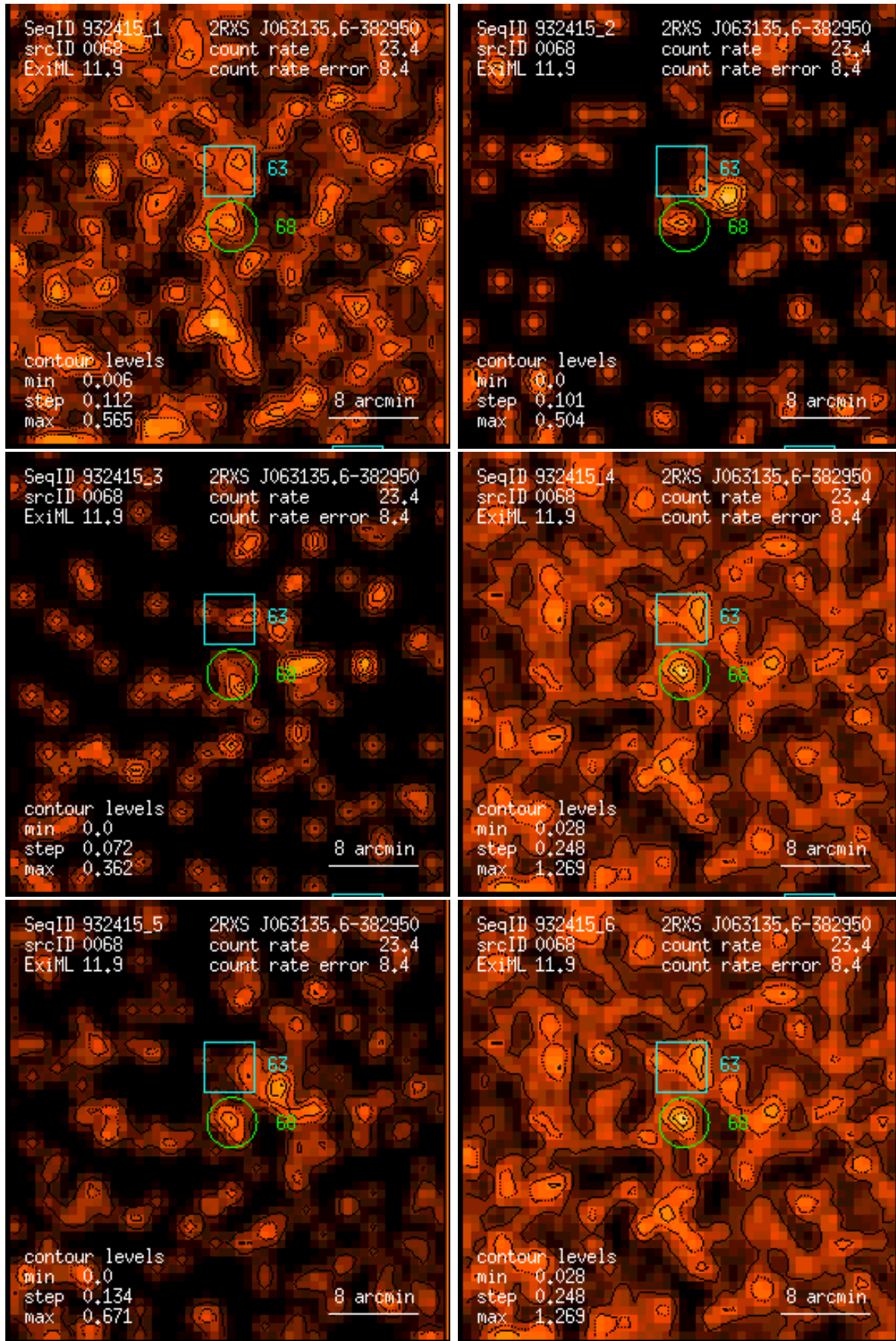
Figure 68: RASS 932415: detection 0068: band rate images, Gaussian filter: (1) PSPC channels 11 – 41, (2) 52 – 90, (3) 91 – 201, (4) 11 – 235, (5) 52 – 201, (6) 11 – 201. Broad band rates in counts/ks. Band rate contour levels in counts/ks/arcmin 2 .
