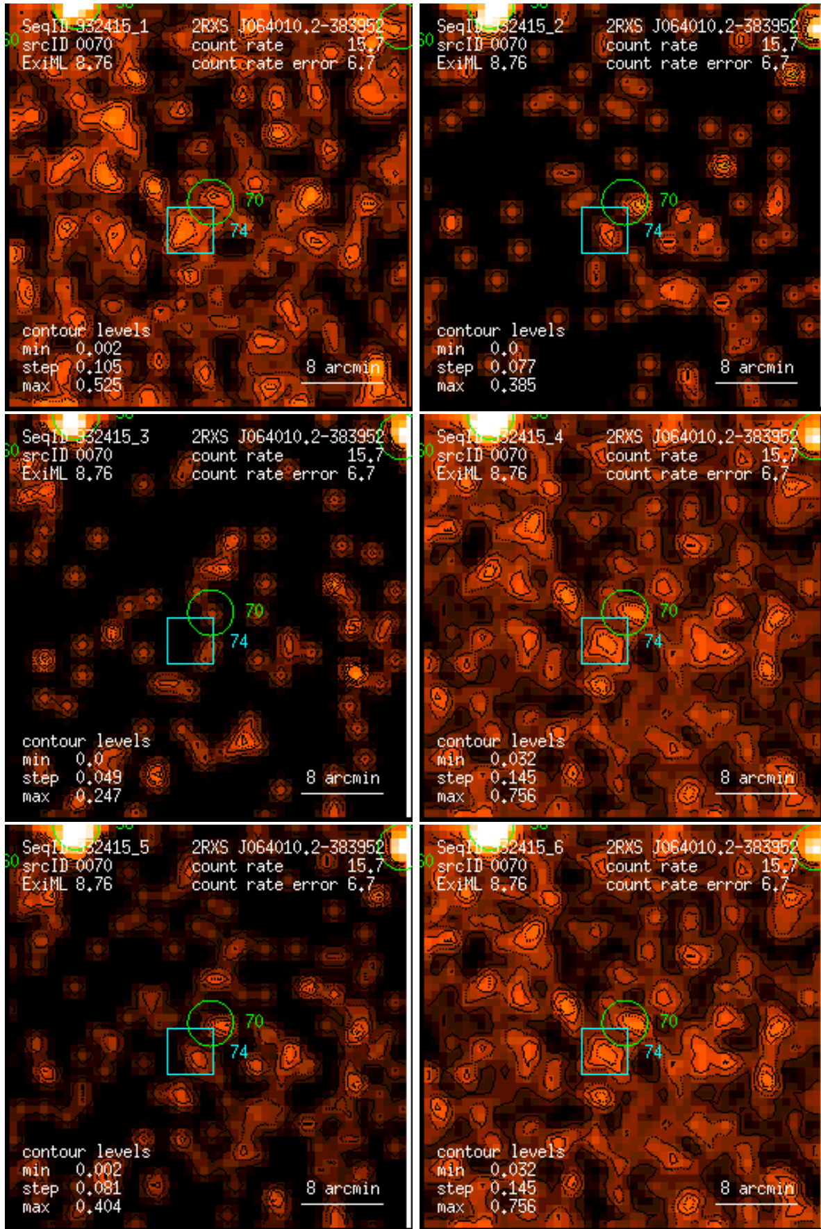
Figure 70: RASS 932415: detection 0070: band rate images, Gaussian filter: (1) PSPC channels 11 – 41, (2) 52 – 90, (3) 91 – 201, (4) 11 – 235, (5) 52 – 201, (6) 11 – 201. Broad band rates in counts/ks. Band rate contour levels in counts/ks/arcmin 2 .
