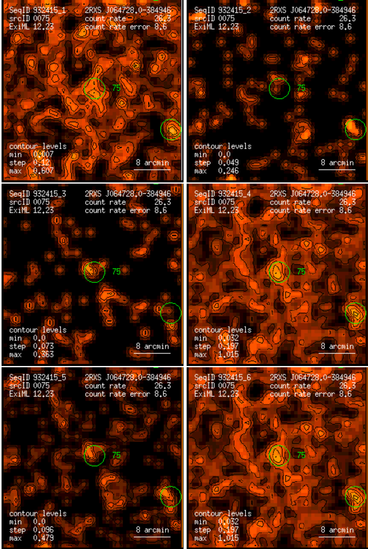
Figure 75: RASS 932415: detection 0075: band rate images, Gaussian filter: (1) PSPC channels 11 – 41, (2) 52 – 90, (3) 91 – 201, (4) 11 – 235, (5) 52 – 201, (6) 11 – 201. Broad band rates in counts/ks. Band rate contour levels in counts/ks/arcmin 2 .
