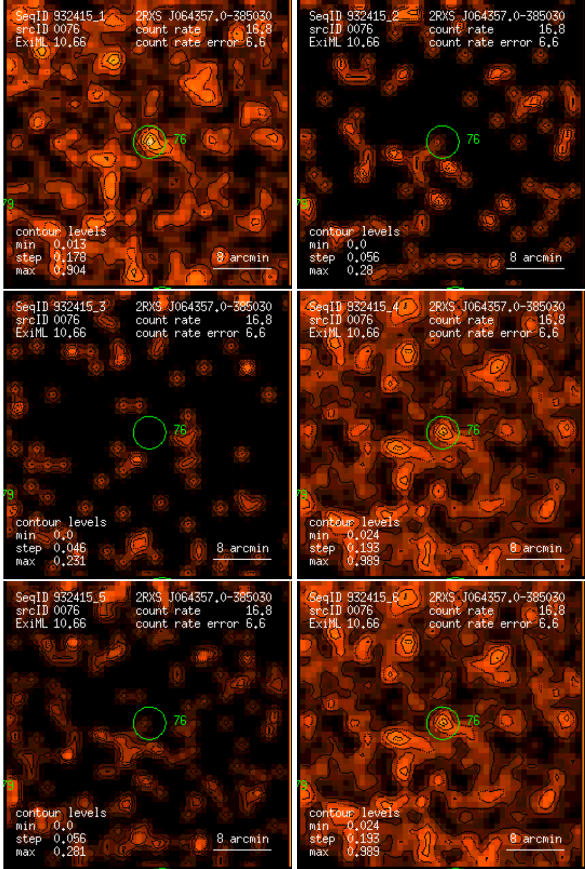
Figure 76: RASS 932415: detection 0076: band rate images, Gaussian filter: (1) PSPC channels 11 – 41, (2) 52 – 90, (3) 91 – 201, (4) 11 – 235, (5) 52 – 201, (6) 11 – 201. Broad band rates in counts/ks. Band rate contour levels in counts/ks/arcmin 2 .
