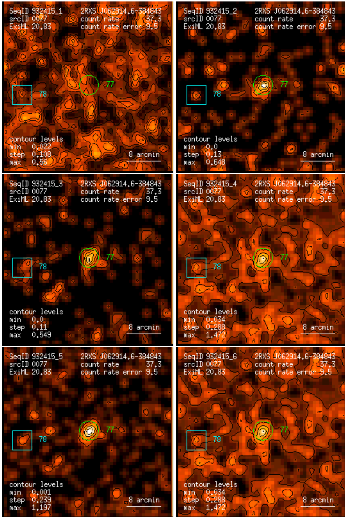
Figure 77: RASS 932415: detection 0077: band rate images, Gaussian filter: (1) PSPC channels 11 – 41, (2) 52 – 90, (3) 91 – 201, (4) 11 – 235, (5) 52 – 201, (6) 11 – 201. Broad band rates in counts/ks. Band rate contour levels in counts/ks/arcmin 2 .
