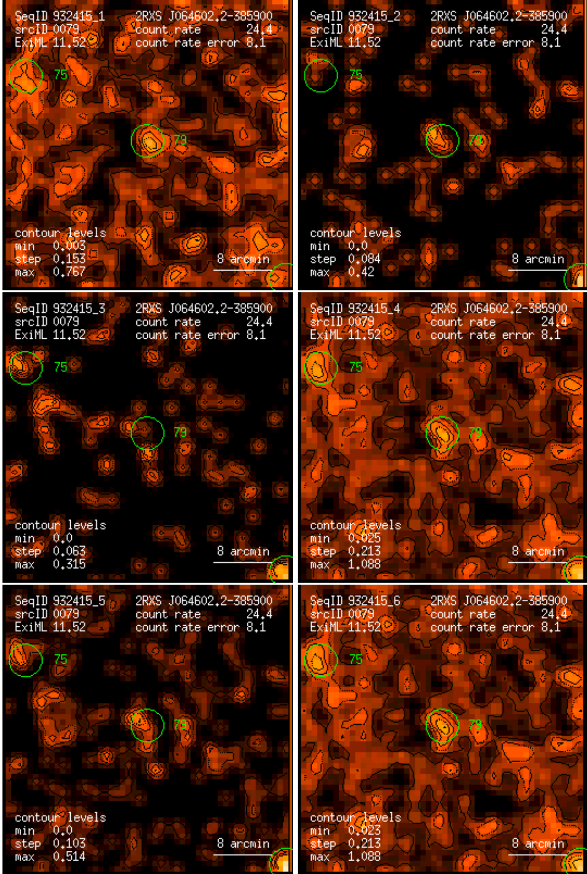
Figure 79: RASS 932415: detection 0079: band rate images, Gaussian filter: (1) PSPC channels 11 – 41, (2) 52 – 90, (3) 91 – 201, (4) 11 – 235, (5) 52 – 201, (6) 11 – 201. Broad band rates in counts/ks. Band rate contour levels in counts/ks/arcmin 2 .
