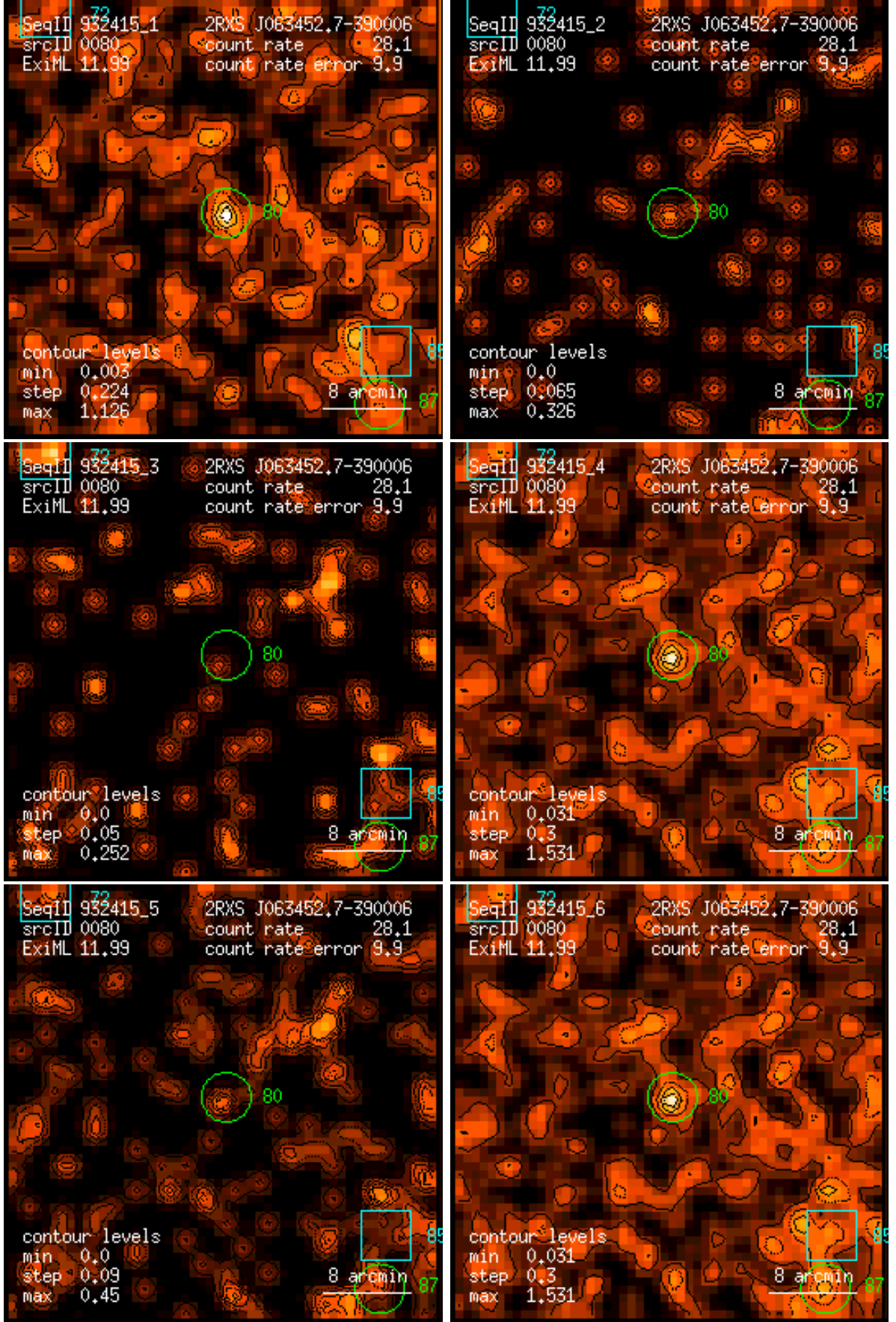
Figure 80: RASS 932415: detection 0080: band rate images, Gaussian filter: (1) PSPC channels 11 – 41, (2) 52 – 90, (3) 91 – 201, (4) 11 – 235, (5) 52 – 201, (6) 11 – 201. Broad band rates in counts/ks. Band rate contour levels in counts/ks/arcmin 2 .
