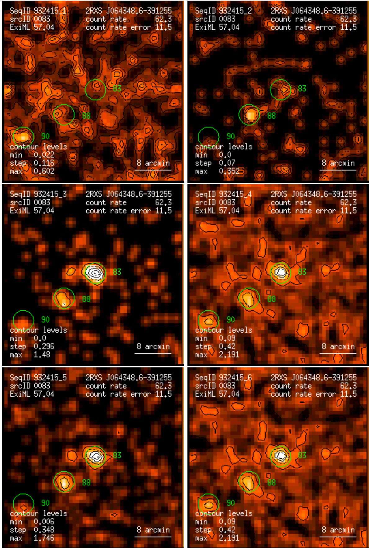
Figure 83: RASS 932415: detection 0083: band rate images, Gaussian filter: (1) PSPC channels 11 – 41, (2) 52 – 90, (3) 91 – 201, (4) 11 – 235, (5) 52 – 201, (6) 11 – 201. Broad band rates in counts/ks. Band rate contour levels in counts/ks/arcmin 2 .
