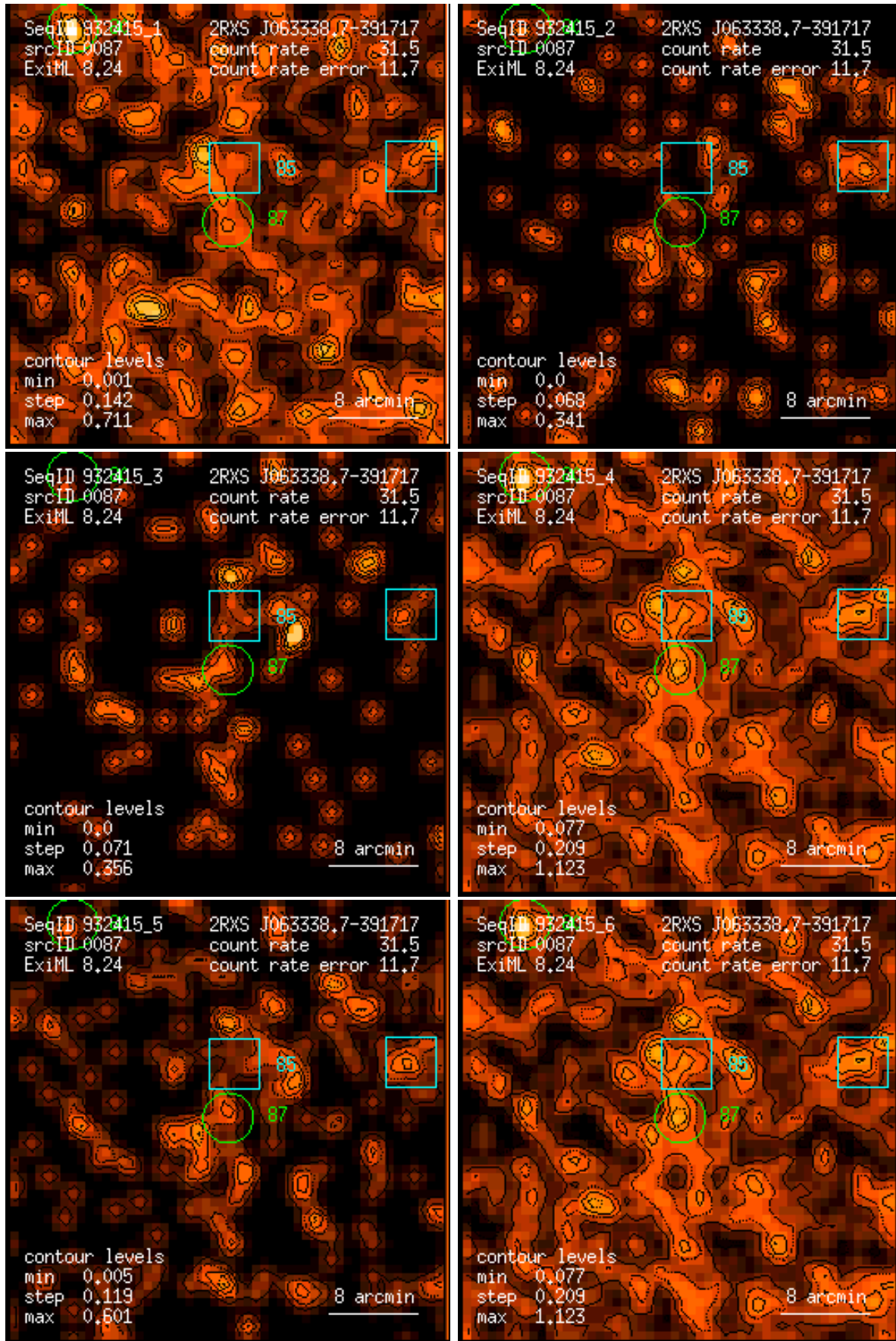
Figure 87: RASS 932415: detection 0087: band rate images, Gaussian filter: (1) PSPC channels 11 – 41, (2) 52 – 90, (3) 91 – 201, (4) 11 – 235, (5) 52 – 201, (6) 11 – 201. Broad band rates in counts/ks. Band rate contour levels in counts/ks/arcmin 2 .
