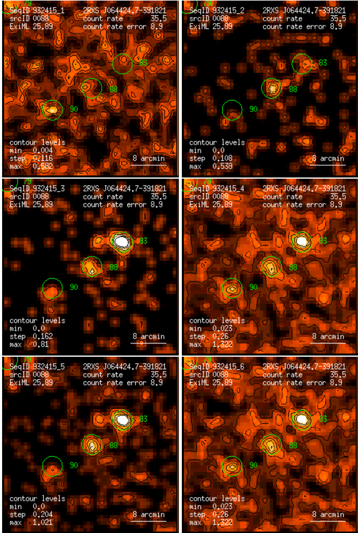
Figure 88: RASS 932415: detection 0088: band rate images, Gaussian filter: (1) PSPC channels 11 – 41, (2) 52 – 90, (3) 91 – 201, (4) 11 – 235, (5) 52 – 201, (6) 11 – 201. Broad band rates in counts/ks. Band rate contour levels in counts/ks/arcmin 2 .
