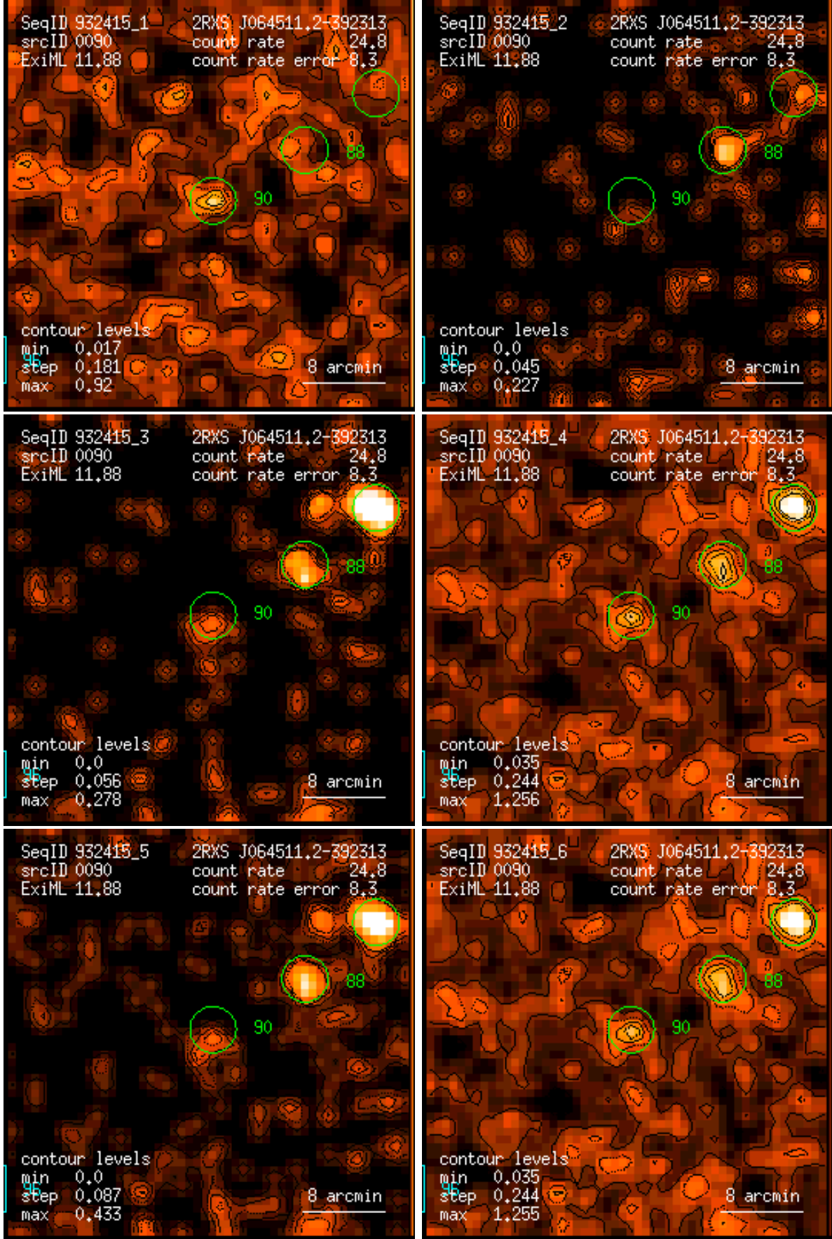
Figure 90: RASS 932415: detection 0090: band rate images, Gaussian filter: (1) PSPC channels 11 – 41, (2) 52 – 90, (3) 91 – 201, (4) 11 – 235, (5) 52 – 201, (6) 11 – 201. Broad band rates in counts/ks. Band rate contour levels in counts/ks/arcmin 2 .
