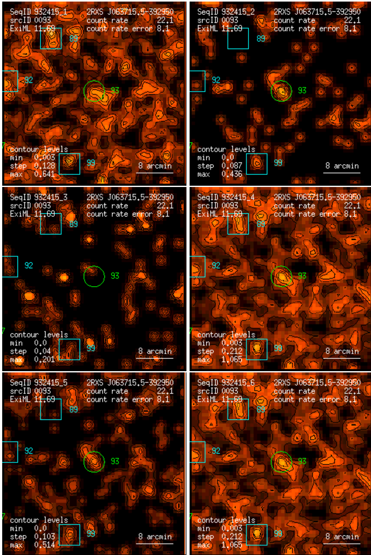
Figure 93: RASS 932415: detection 0093: band rate images, Gaussian filter: (1) PSPC channels 11 – 41, (2) 52 – 90, (3) 91 – 201, (4) 11 – 235, (5) 52 – 201, (6) 11 – 201. Broad band rates in counts/ks. Band rate contour levels in counts/ks/arcmin 2 .
