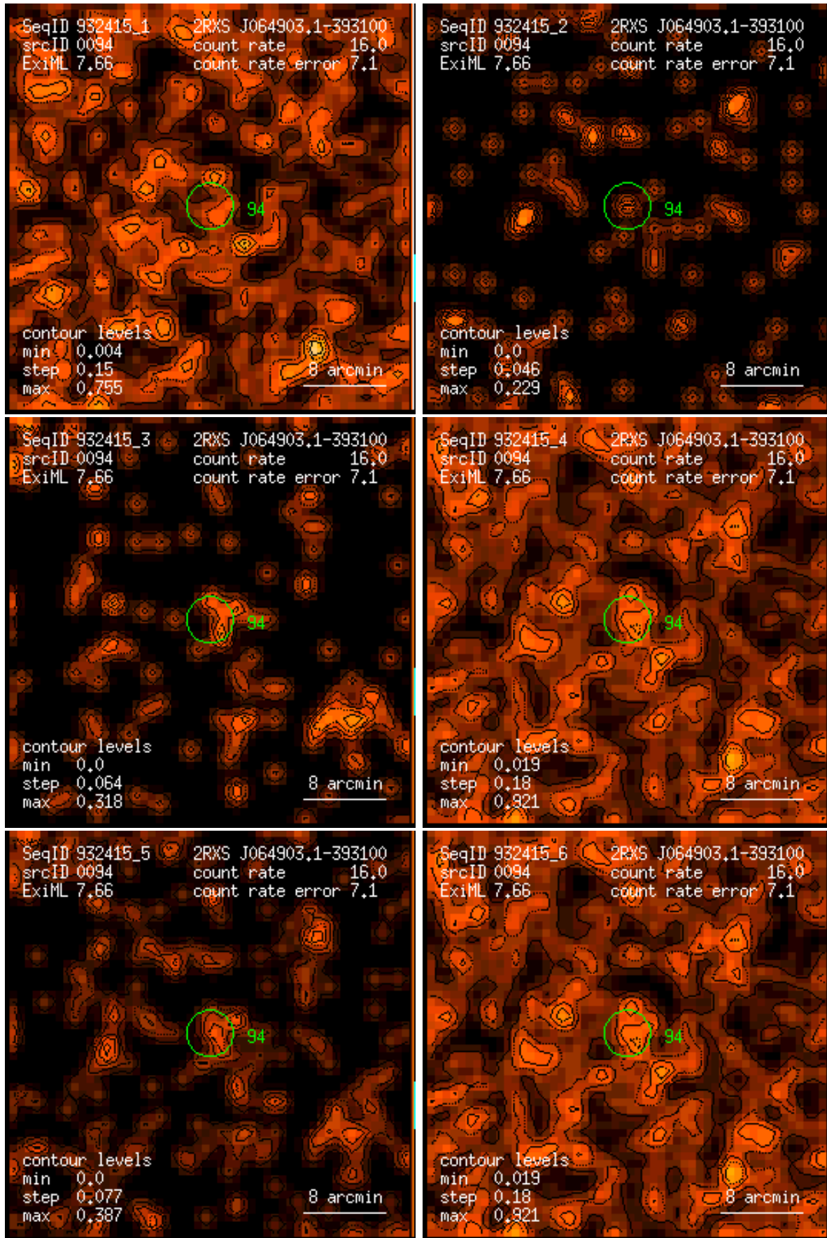
Figure 94: RASS 932415: detection 0094: band rate images, Gaussian filter: (1) PSPC channels 11 – 41, (2) 52 – 90, (3) 91 – 201, (4) 11 – 235, (5) 52 – 201, (6) 11 – 201. Broad band rates in counts/ks. Band rate contour levels in counts/ks/arcmin 2 .
