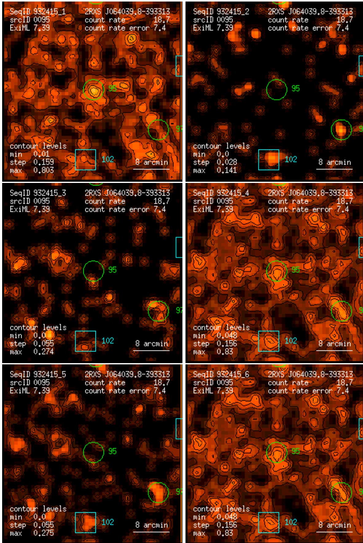
Figure 95: RASS 932415: detection 0095: band rate images, Gaussian filter: (1) PSPC channels 11 – 41, (2) 52 – 90, (3) 91 – 201, (4) 11 – 235, (5) 52 – 201, (6) 11 – 201. Broad band rates in counts/ks. Band rate contour levels in counts/ks/arcmin 2 .
