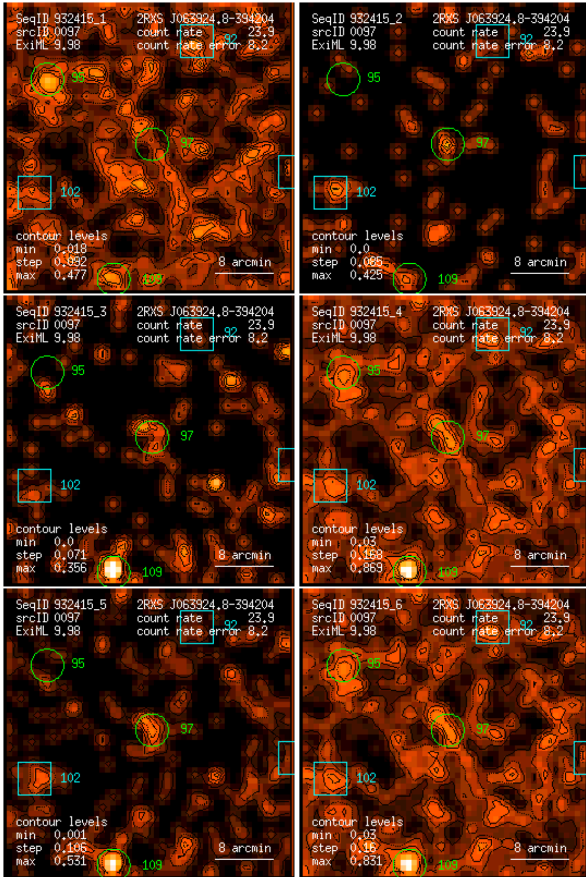
Figure 97: RASS 932415: detection 0097: band rate images, Gaussian filter: (1) PSPC channels 11 – 41, (2) 52 – 90, (3) 91 – 201, (4) 11 – 235, (5) 52 – 201, (6) 11 – 201. Broad band rates in counts/ks. Band rate contour levels in counts/ks/arcmin 2 .
