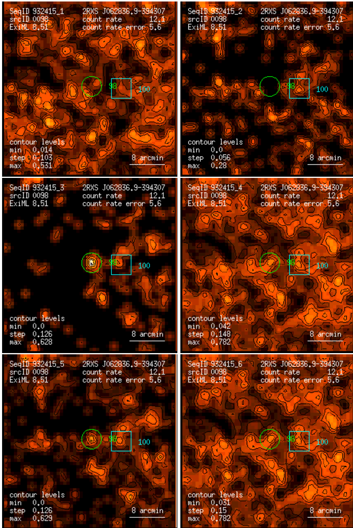
Figure 98: RASS 932415: detection 0098: band rate images, Gaussian filter: (1) PSPC channels 11 – 41, (2) 52 – 90, (3) 91 – 201, (4) 11 – 235, (5) 52 – 201, (6) 11 – 201. Broad band rates in counts/ks. Band rate contour levels in counts/ks/arcmin 2 .
