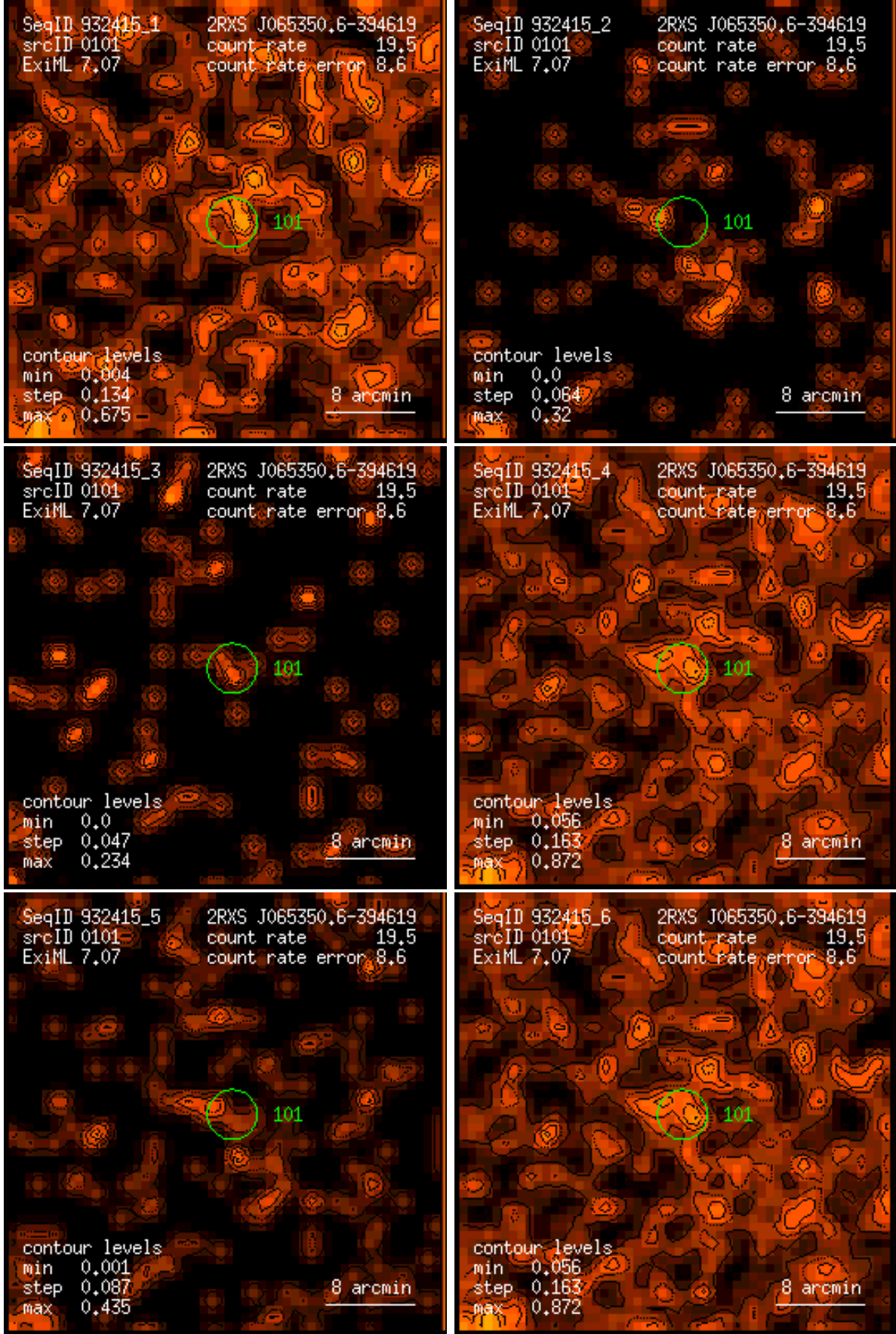
Figure 101: RASS 932415: detection 0101: band rate images, Gaussian filter: (1) PSPC channels 11 – 41, (2) 52 – 90, (3) 91 – 201, (4) 11 – 235, (5) 52 – 201, (6) 11 – 201. Broad band rates in counts/ks. Band rate contour levels in counts/ks/arcmin 2 .
