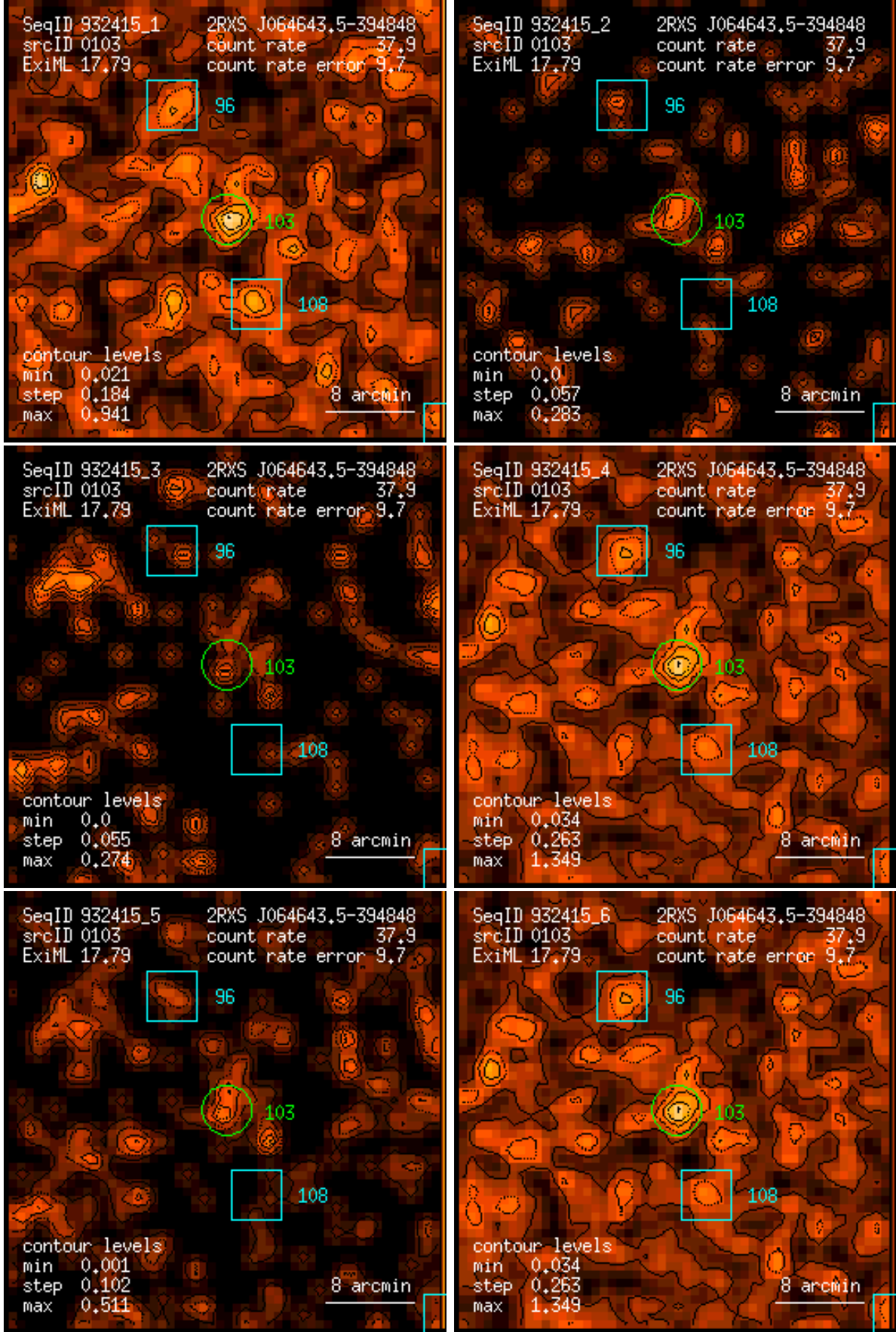
Figure 103: RASS 932415: detection 0103: band rate images, Gaussian filter: (1) PSPC channels 11 – 41, (2) 52 – 90, (3) 91 – 201, (4) 11 – 235, (5) 52 – 201, (6) 11 – 201. Broad band rates in counts/ks. Band rate contour levels in counts/ks/arcmin 2 .
