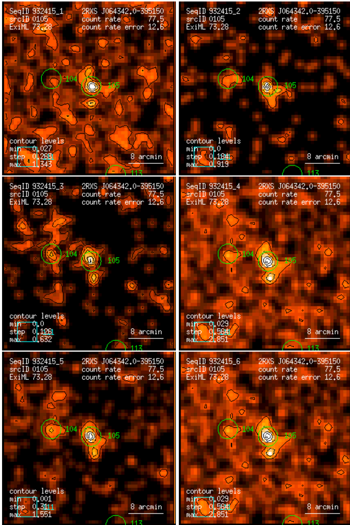
Figure 105: RASS 932415: detection 0105: band rate images, Gaussian filter: (1) PSPC channels 11 – 41, (2) 52 – 90, (3) 91 – 201, (4) 11 – 235, (5) 52 – 201, (6) 11 – 201. Broad band rates in counts/ks. Band rate contour levels in counts/ks/arcmin 2 .
