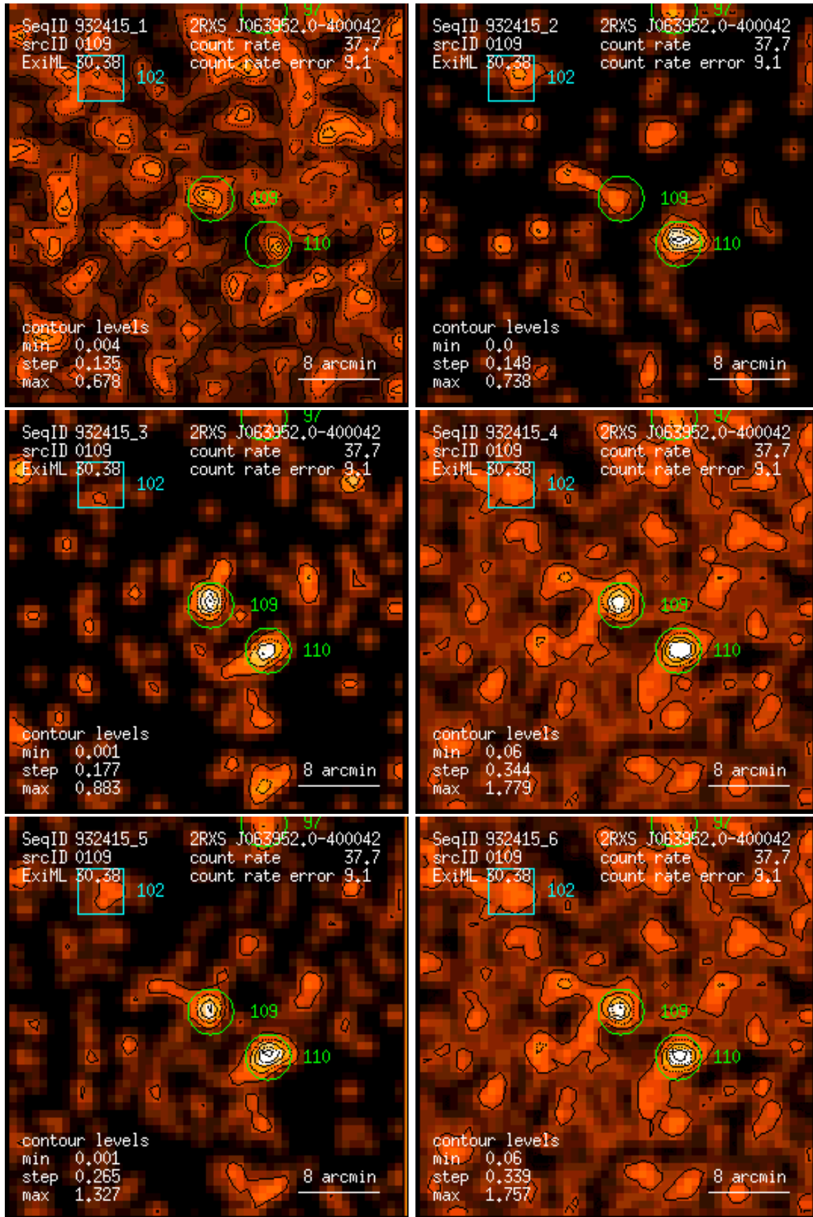
Figure 109: RASS 932415: detection 0109: band rate images, Gaussian filter: (1) PSPC channels 11 – 41, (2) 52 – 90, (3) 91 – 201, (4) 11 – 235, (5) 52 – 201, (6) 11 – 201. Broad band rates in counts/ks. Band rate contour levels in counts/ks/arcmin 2 .
