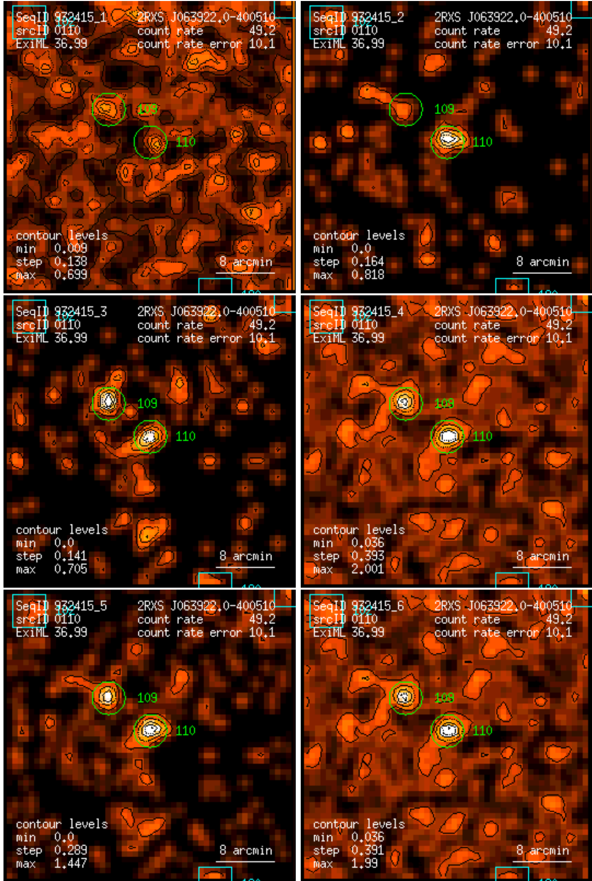
Figure 110: RASS 932415: detection 0110: band rate images, Gaussian filter: (1) PSPC channels 11 – 41, (2) 52 – 90, (3) 91 – 201, (4) 11 – 235, (5) 52 – 201, (6) 11 – 201. Broad band rates in counts/ks. Band rate contour levels in counts/ks/arcmin 2 .
