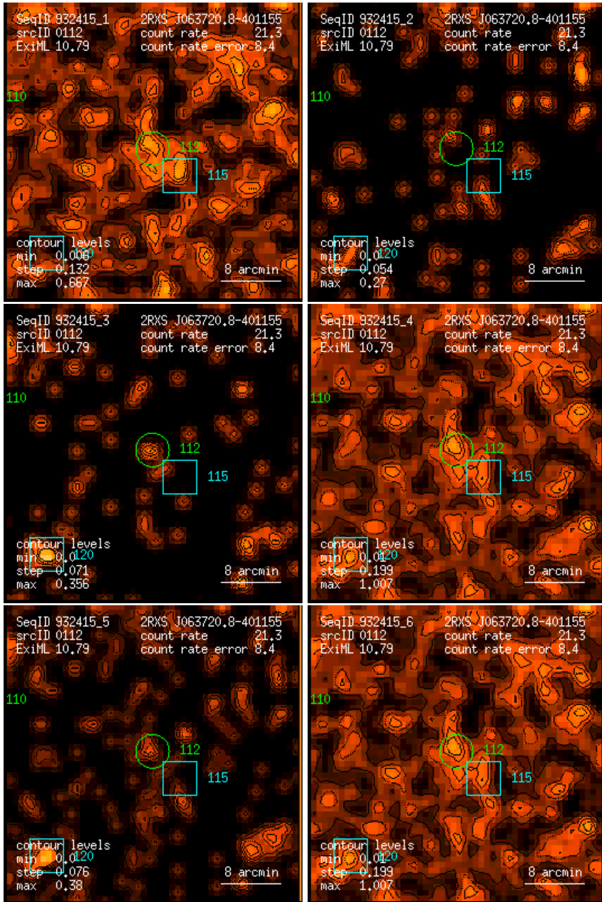
Figure 112: RASS 932415: detection 0112: band rate images, Gaussian filter: (1) PSPC channels 11 – 41, (2) 52 – 90, (3) 91 – 201, (4) 11 – 235, (5) 52 – 201, (6) 11 – 201. Broad band rates in counts/ks. Band rate contour levels in counts/ks/arcmin 2 .
