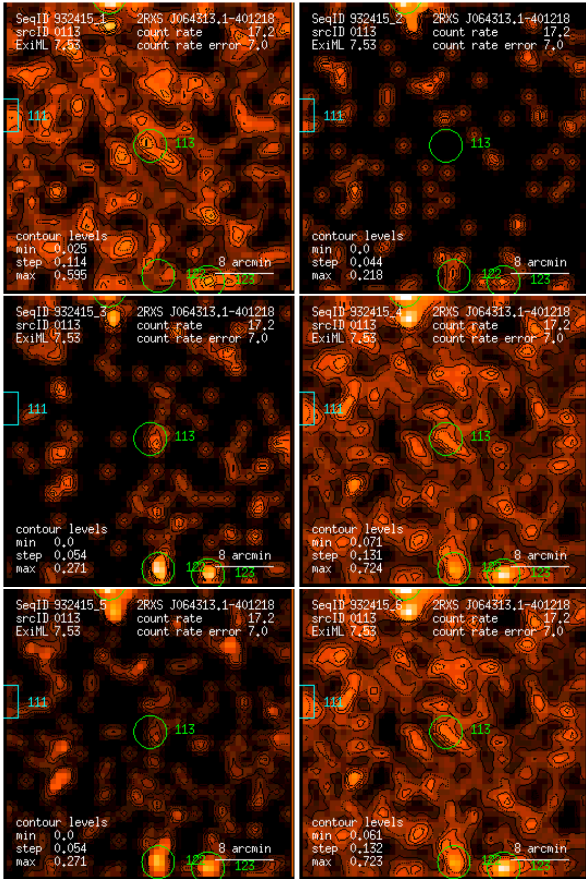
Figure 113: RASS 932415: detection 0113: band rate images, Gaussian filter: (1) PSPC channels 11 – 41, (2) 52 – 90, (3) 91 – 201, (4) 11 – 235, (5) 52 – 201, (6) 11 – 201. Broad band rates in counts/ks. Band rate contour levels in counts/ks/arcmin 2 .
