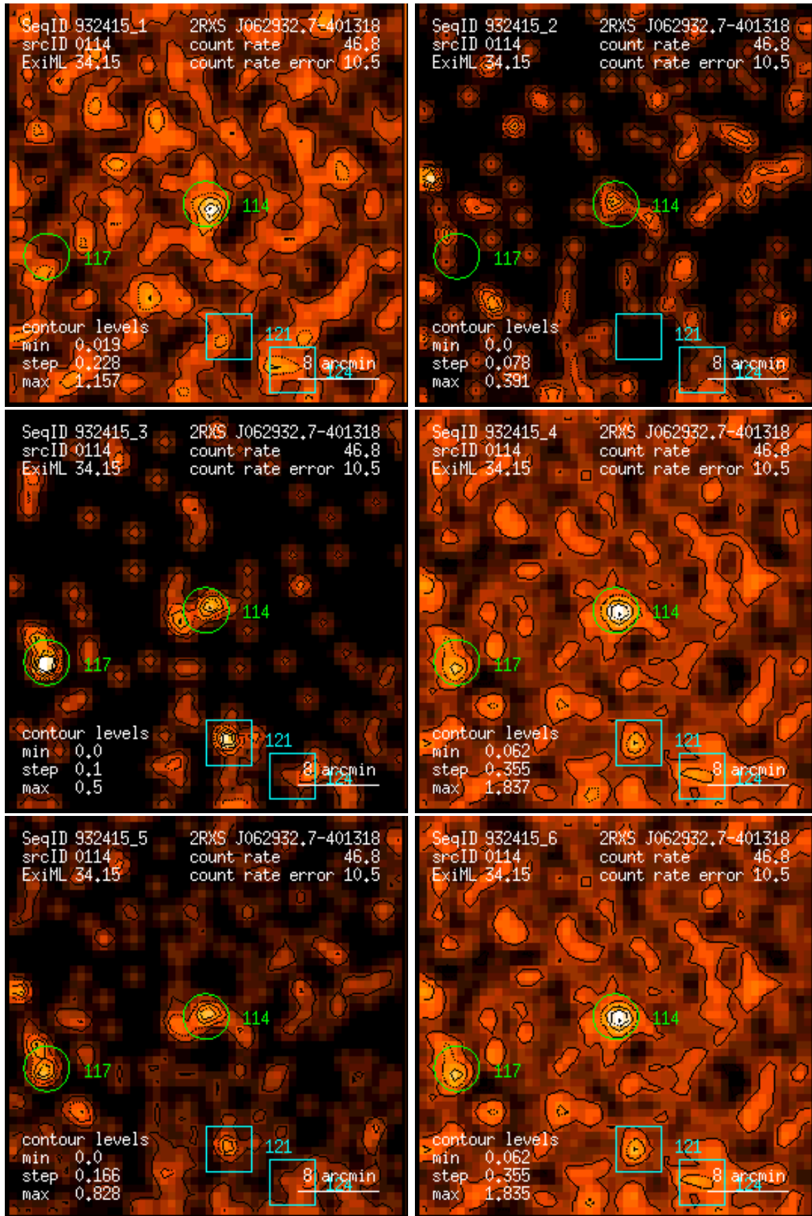
Figure 114: RASS 932415: detection 0114: band rate images, Gaussian filter: (1) PSPC channels 11 – 41, (2) 52 – 90, (3) 91 – 201, (4) 11 – 235, (5) 52 – 201, (6) 11 – 201. Broad band rates in counts/ks. Band rate contour levels in counts/ks/arcmin 2 .
