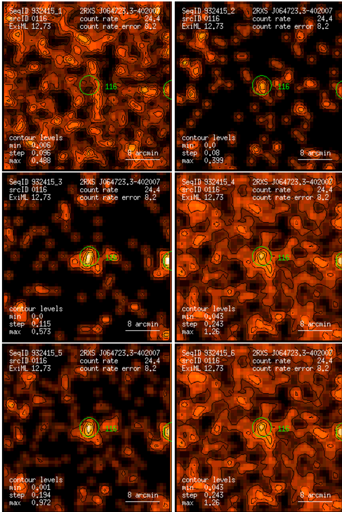
Figure 116: RASS 932415: detection 0116: band rate images, Gaussian filter: (1) PSPC channels 11 – 41, (2) 52 – 90, (3) 91 – 201, (4) 11 – 235, (5) 52 – 201, (6) 11 – 201. Broad band rates in counts/ks. Band rate contour levels in counts/ks/arcmin 2 .
