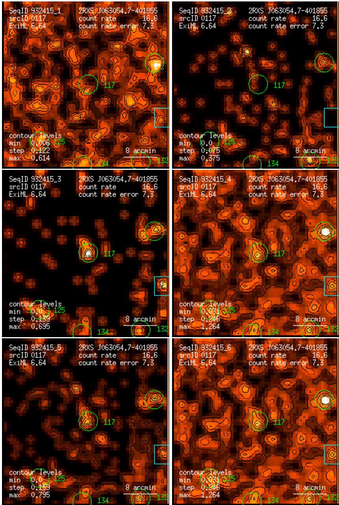
Figure 117: RASS 932415: detection 0117: band rate images, Gaussian filter: (1) PSPC channels 11 – 41, (2) 52 – 90, (3) 91 – 201, (4) 11 – 235, (5) 52 – 201, (6) 11 – 201. Broad band rates in counts/ks. Band rate contour levels in counts/ks/arcmin 2 .
