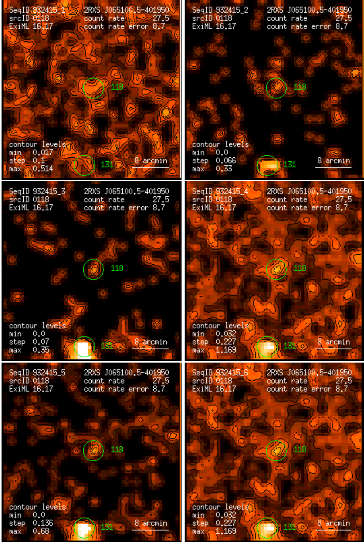
Figure 118: RASS 932415: detection 0118: band rate images, Gaussian filter: (1) PSPC channels 11 – 41, (2) 52 – 90, (3) 91 – 201, (4) 11 – 235, (5) 52 – 201, (6) 11 – 201. Broad band rates in counts/ks. Band rate contour levels in counts/ks/arcmin 2 .
