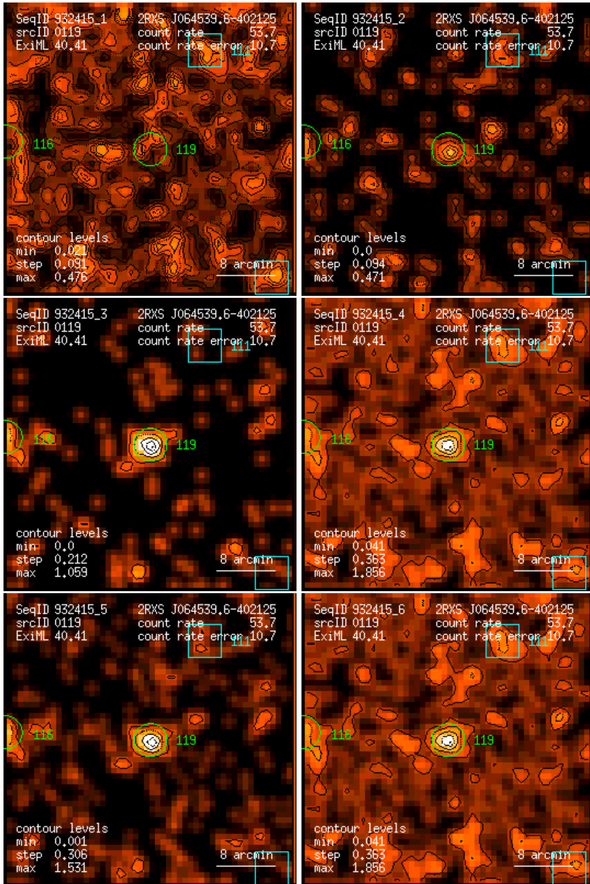
Figure 119: RASS 932415: detection 0119: band rate images, Gaussian filter: (1) PSPC channels 11 – 41, (2) 52 – 90, (3) 91 – 201, (4) 11 – 235, (5) 52 – 201, (6) 11 – 201. Broad band rates in counts/ks. Band rate contour levels in counts/ks/arcmin 2 .
