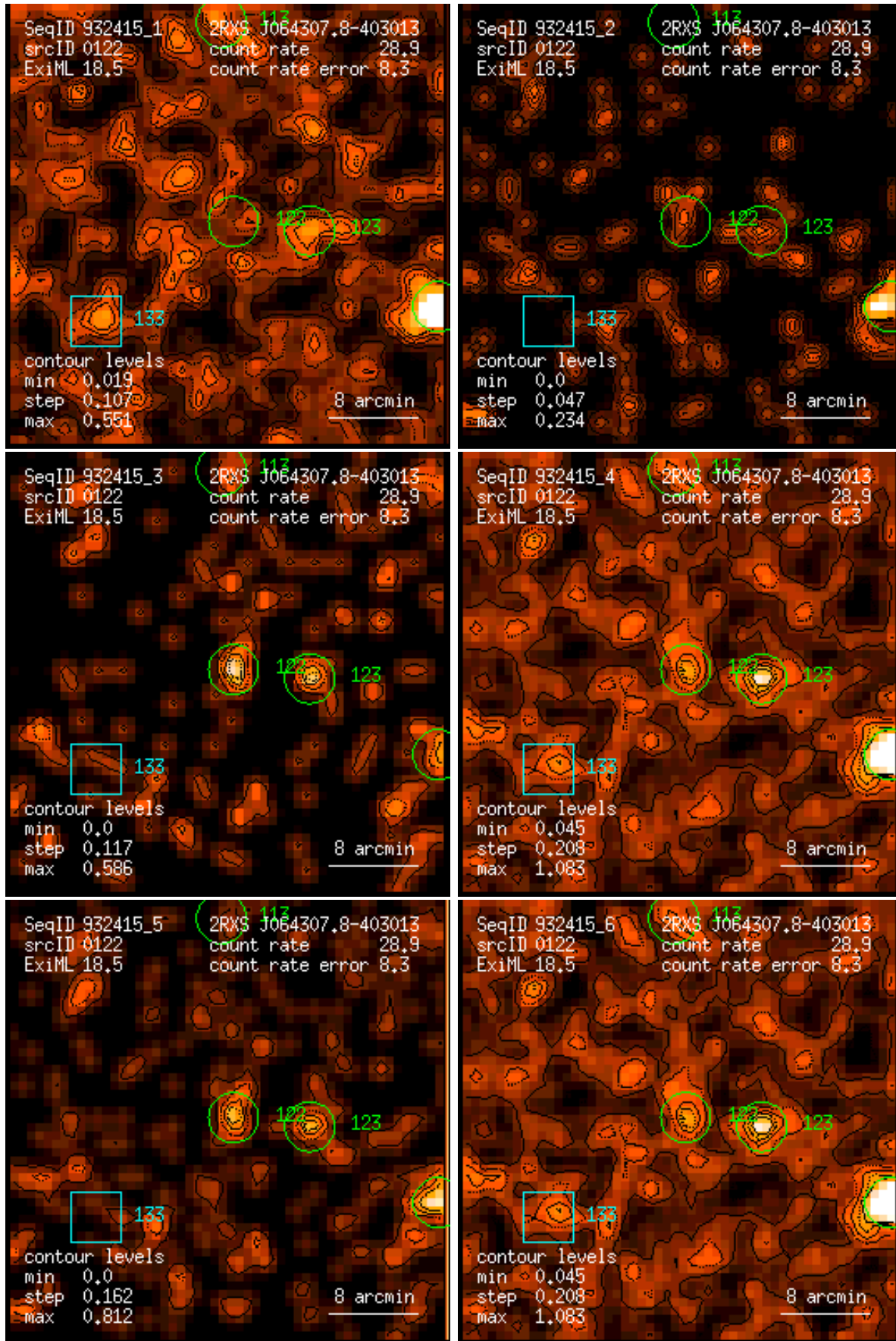
Figure 122: RASS 932415: detection 0122: band rate images, Gaussian filter: (1) PSPC channels 11 – 41, (2) 52 – 90, (3) 91 – 201, (4) 11 – 235, (5) 52 – 201, (6) 11 – 201. Broad band rates in counts/ks. Band rate contour levels in counts/ks/arcmin 2 .
