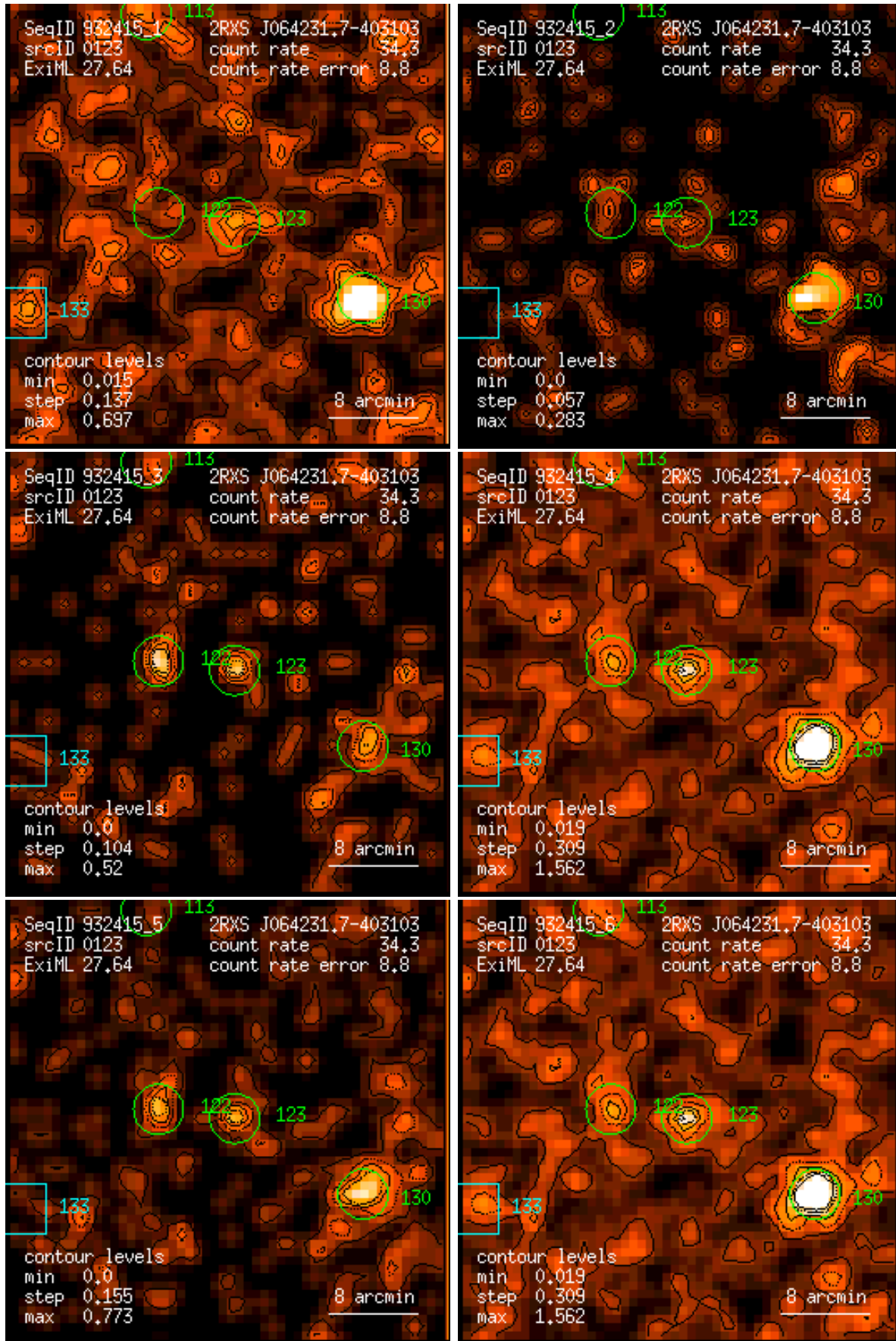
Figure 123: RASS 932415: detection 0123: band rate images, Gaussian filter: (1) PSPC channels 11 – 41, (2) 52 – 90, (3) 91 – 201, (4) 11 – 235, (5) 52 – 201, (6) 11 – 201. Broad band rates in counts/ks. Band rate contour levels in counts/ks/arcmin 2 .
