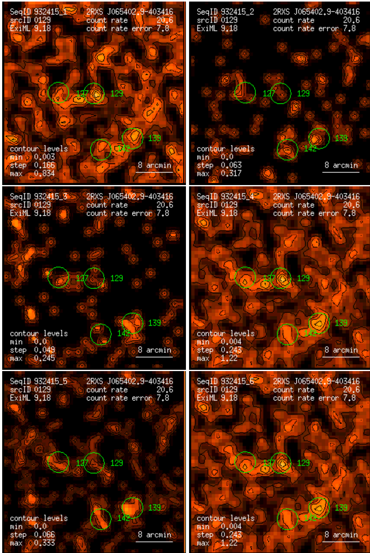
Figure 129: RASS 932415: detection 0129: band rate images, Gaussian filter: (1) PSPC channels 11 – 41, (2) 52 – 90, (3) 91 – 201, (4) 11 – 235, (5) 52 – 201, (6) 11 – 201. Broad band rates in counts/ks. Band rate contour levels in counts/ks/arcmin 2 .
