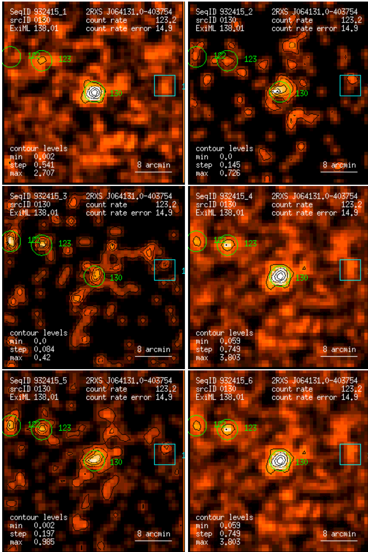
Figure 130: RASS 932415: detection 0130: band rate images, Gaussian filter: (1) PSPC channels 11 – 41, (2) 52 – 90, (3) 91 – 201, (4) 11 – 235, (5) 52 – 201, (6) 11 – 201. Broad band rates in counts/ks. Band rate contour levels in counts/ks/arcmin 2 .
