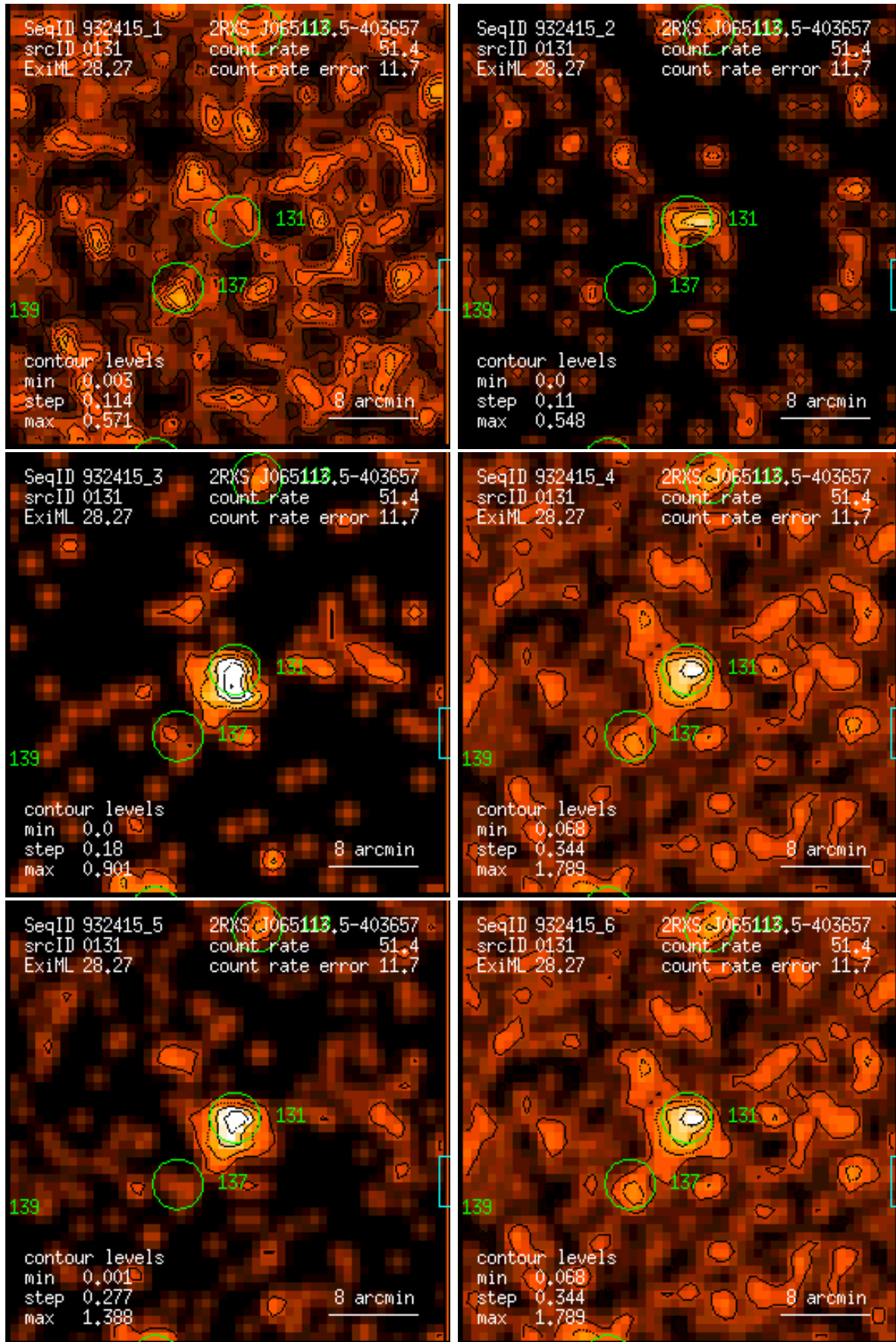
Figure 131: RASS 932415: detection 0131: band rate images, Gaussian filter: (1) PSPC channels 11 – 41, (2) 52 – 90, (3) 91 – 201, (4) 11 – 235, (5) 52 – 201, (6) 11 – 201. Broad band rates in counts/ks. Band rate contour levels in counts/ks/arcmin 2 .
