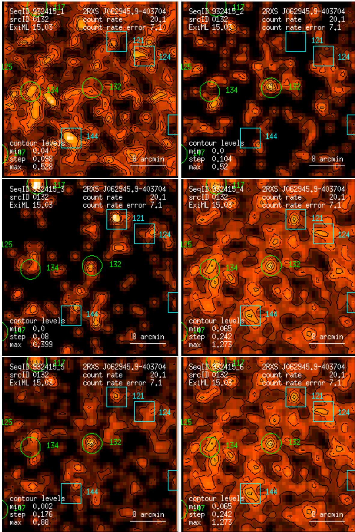
Figure 132: RASS 932415: detection 0132: band rate images, Gaussian filter: (1) PSPC channels 11 – 41, (2) 52 – 90, (3) 91 – 201, (4) 11 – 235, (5) 52 – 201, (6) 11 – 201. Broad band rates in counts/ks. Band rate contour levels in counts/ks/arcmin 2 .
